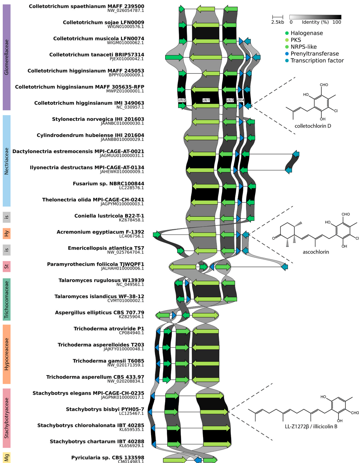
Fig. 4. Conservation and microsynteny of the Colletochlorin (ctc) biosynthetic genes cluster in fungi. In Colletotrichum higginsianum IMI 349063A, this BGC was initially predicted to be a single BGC16 but actually comprises the dpch (Higginsianins) and ctc BGCs located side-by-side. Genes are color-coded according to their putative or experimentally-confirmed functions. The intensity of grey/black shading represents the percentage of amino acid identity. Experimentally-verified BGCs are shown with one of their molecular products. Hy, Hypocreaceae; is, incertae sedis; Mg, Magnaporthaceae; St, Stachybotryaceae.
