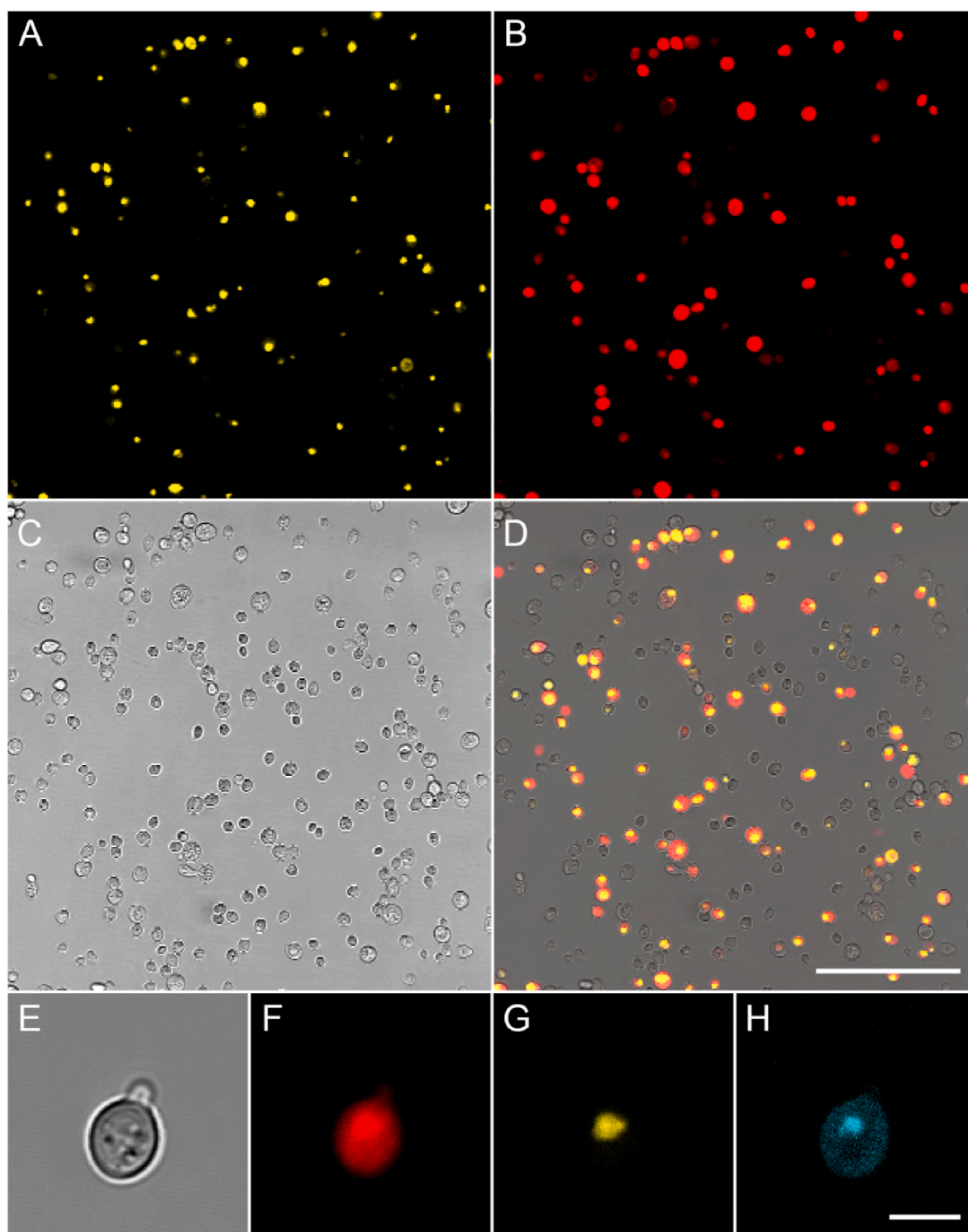
Fig. 2. Confocal microscopy of the yeast strain BJNBC-003 expressing Venus-NLS and mScarlet-I fluorescent proteins and stained with DAPI to detect DNA. A-D, Bar = 50 \mu m. E-H, from left to right, bright-field image showing the yeast cells, red fluorescence corresponding to mScarlet-I, yellow fluorescence corresponding to Venus and, blue fluorescence corresponding to DAPI. The mScarlet-I signal is distributed throughout the cell whereas the Venus signal is co-localized with DNA in the nucleus. Bar = 5 \mu m.
