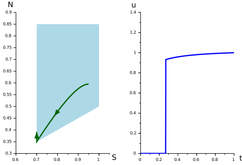
Figure 6: Optimal solution for N_0 = N_0^b
