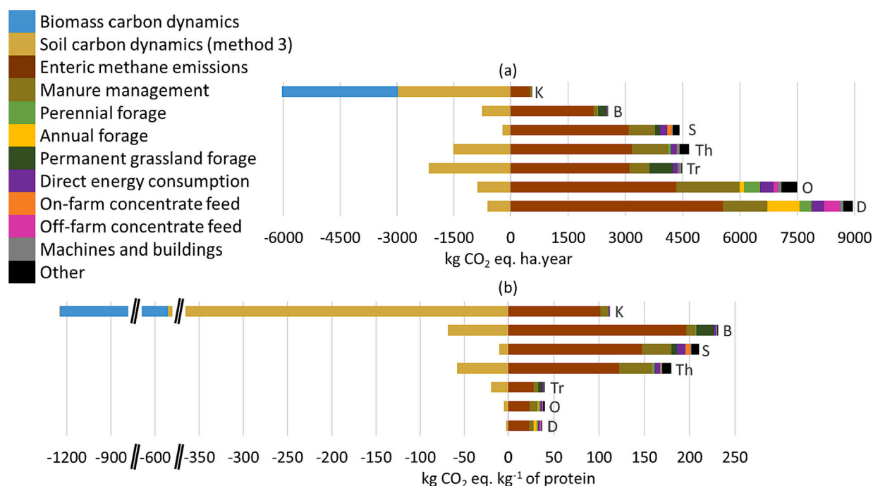
Fig. 3. Contribution analysis for the climate change impact of the seven systems (K: Knepp, B: La Barge, S: Saint Laurent de la Prée, Th: Thorigné d'Anjou, Tr: Trévarn, O: Oasys, D: Dervall) per (a) ha and (b) kg of human-edible animal protein. To increase readability of the graphs, the contributions of soil carbon dynamics shown (always negative) are only those calculated according to method 3 (Poeplau et al. (2011) and Pellerin et al. (2019)). See Table S11 for detailed results of methods 2 (Pellerin et al. (2019)) and 3.
