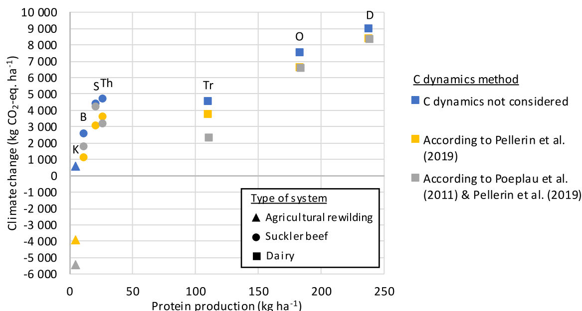
Fig. 4. Climate change impact per ha as a function of human-edible animal protein production per ha of the seven systems (K: Knepp, B: La Barge, S: Saint Laurent de la Prée, Th: Thorigné d'Anjou, Tr: Trévarn, O: Oasys, D: Derval). Colours of symbols identify the three methods used to consider (or not) carbon (C) dynamics in the soil and unharvested woody biomass.
