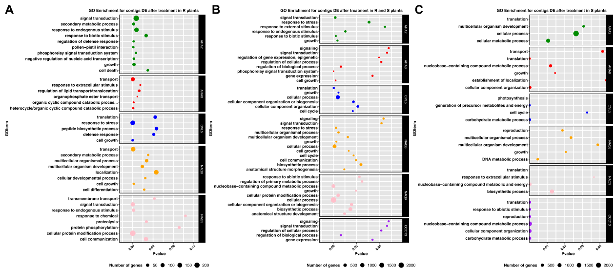
Fig. 3 Result of GO enrichment analysis for genes DE after herbicide application in each phenotype in the six populations studied. The BP terms displayed are significant at the elim-Fisher test ( p -value < 0.05 ) and represent at least 1% of the DE genes in the population of interest. A terms associated with DE genes specific to resistant plants, B terms associated with DE genes shared by resistant and sensitive plants, C terms associated with DE genes specific to sensitive plants
