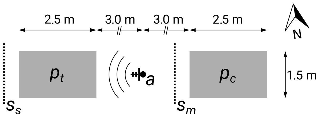
Fig. 1. The experiment setup; symbols used: a – antenna, p_c – control plot, p_t – treatment plot (or “radiation plot”), s_m – electromagnetic shielding screen, s_s – sham screen.
