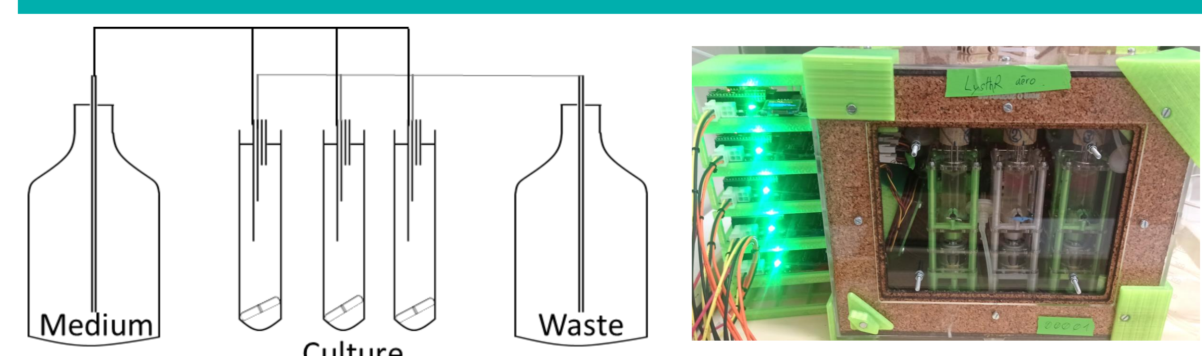
Figure 5: Continuous culturing device developed by Cyprien Guérin and Pierre Nicolas (MalAGE)
