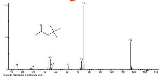
ACETIC ACID
