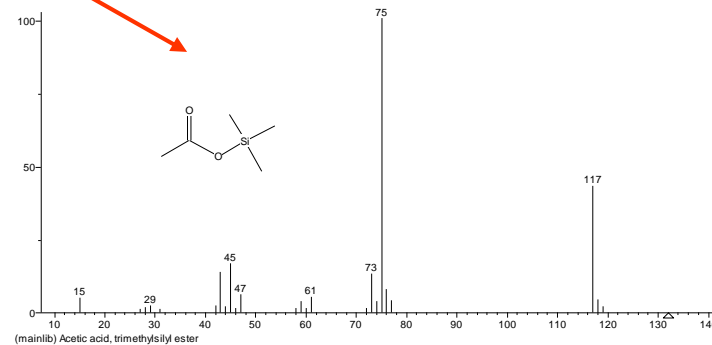
ACETIC ACID
