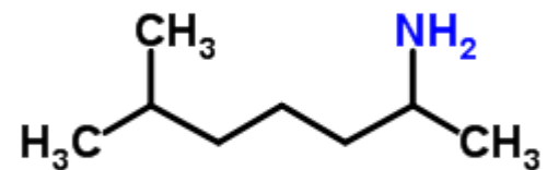
Octodrine
