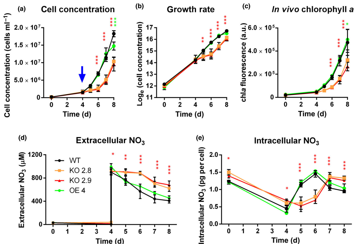
Fig. 4 Growth phenotype in P. tricornutum wild-type (WT) and Ptnpf1 knock-out mutants. (a) Cell concentration, (b) natural logarithm of growth curves and (c) measurement of in vivo chlorophyll a autofluorescence, providing a proxy for growth, for the WT, KO 2.8 and 2.9 knock-out mutants and one OE4 overexpressing strain (d) Extracellular \text{NO}_3^- removed from the media by WT and Ptnpf1 knock-out cells measured by UV spectrophotometry. (e) Intracellular \text{NO}_3^- extracted from cells and measured by UV spectrophotometry. The blue arrow indicates the \text{NO}_3^- repletion day. The values are shown as mean \pm SD ( n = 3 biological replicates). *, P < 0.05 ; **, P < 0.01 ; ***, P < 0.001 resulting from the two-way ANOVA performed.
