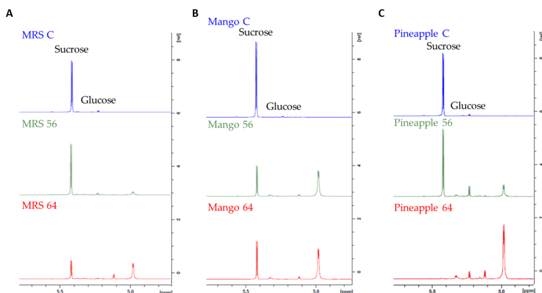
Figure 6. One-dimensional ^1\text{H} NMR spectra in the anomeric region of EPS produced on (A) MRS, (B) mango purée, and (C) pineapple juice media (pH 6, sucrose: 20% for MRS, 9.6% for pineapple juice and 3.25% for mango purée). C: sterile medium, 56: L. pseudomesenteroides strain 56, 64: W. cibaria strain 64.
