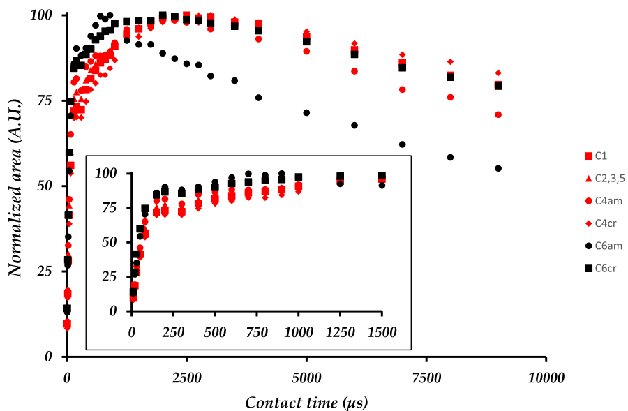
Fig. 4. Normalized area of each CNC carbon relative to contact time. The insert shows the signal evolution for short contact times (< 1500 μs). These data were obtained with 512 accumulations and recycling delays of 8 s.
