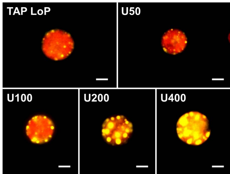
Figure S3: Lipid droplet accumulation in Coelastrella sp. PCV challenged with uranium. Coelastrella sp. PCV was cultivated for 1 day at 21°C in continuous white light (40 \mu E) in TAP LoP containing 50 to 400 \mu M of uranyl nitrate. Cells were stained with Nile Red and imaged using a Zeiss Axioplan 2 microscope. Chlorophyll autofluorescence is in red; lipid droplets stained with Nile Red are in yellow. Scale bar = 5 \mu m.
