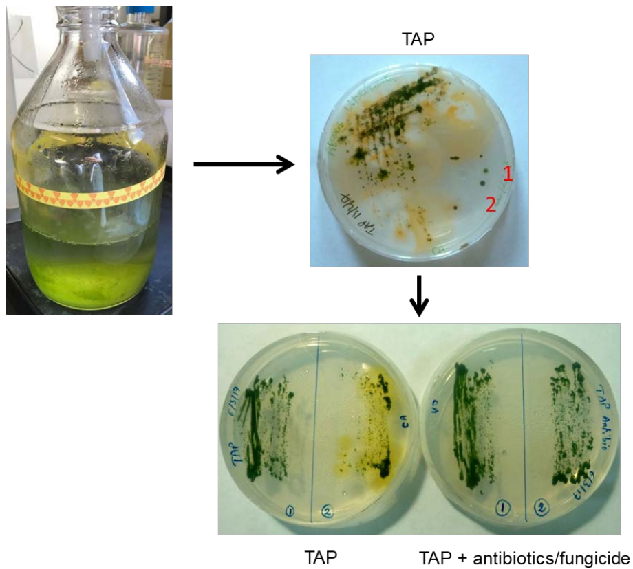
Figure S1: Isolation of Coelastrella sp. PCV from liquid wastes contaminated by uranium. The algal bloom developed in laboratory wastes from plant culture medium contaminated with uranyl nitrate (about 5 \mu M). The original sampling streaked on TAP-agar was contaminated with bacteria and fungi. Single algal colonies (1 and 2) could be cleared of contaminants by two successive rounds of selection on TAP-agar supplemented with antibiotics (ampicillin and cefotaxime) and a broad-spectrum fungicide (carbendazim). Plates were incubated at 21°C in continuous light (20 \mu E) for 7 days.
