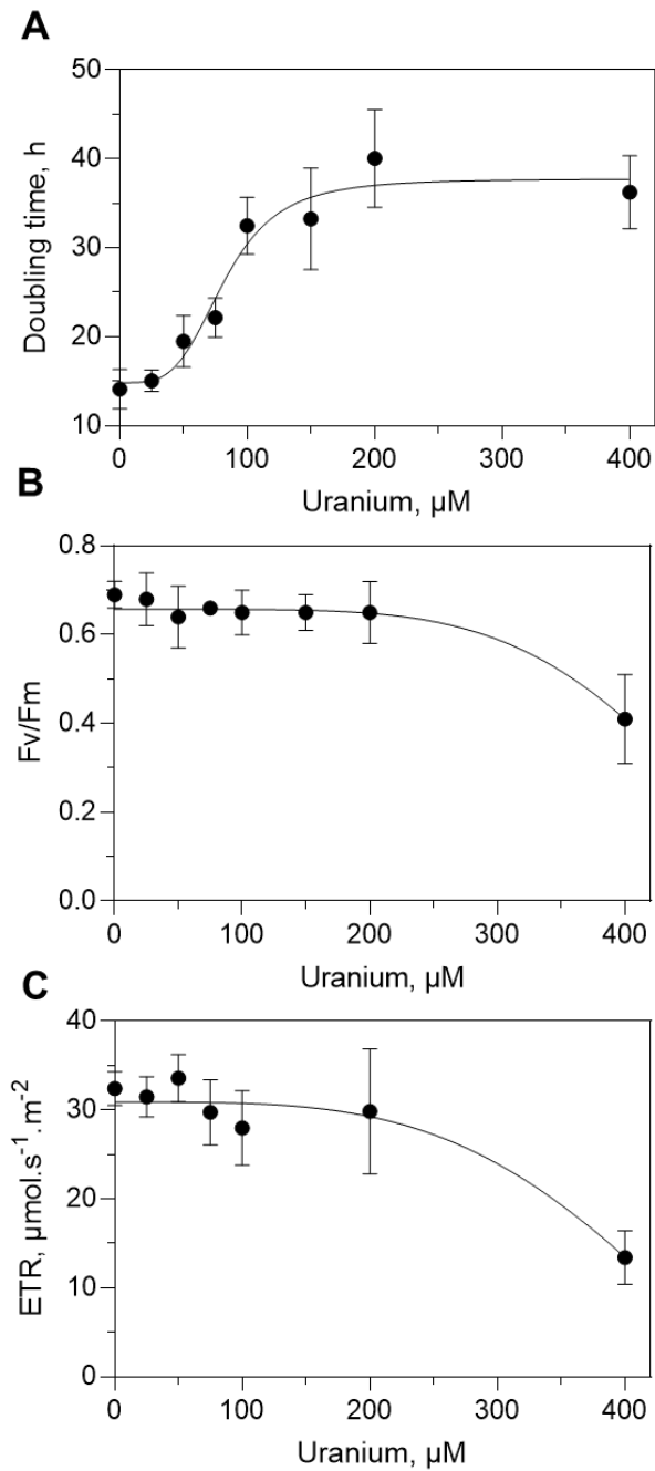
Figure S2: Inhibition of growth and photosynthesis by uranium in Coelastrella sp. PCV .
