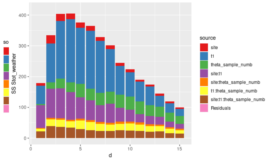
weather
