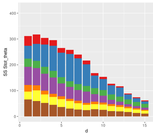
theta
