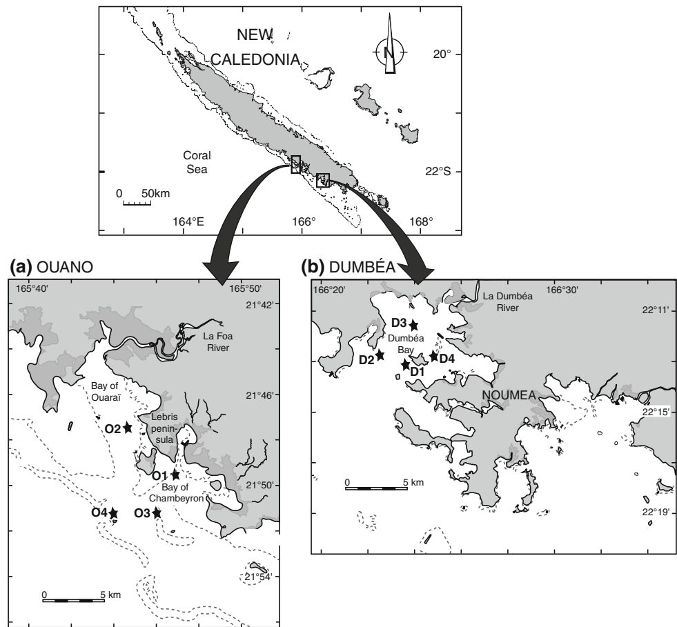
Fig. 1 Position of the sampling stations (stars) at Ouano and Dumbéa, southwestern New Caledonia. Dark grey zones on the maps indicate the mangroves; dotted lines represent the location of coral reefs
