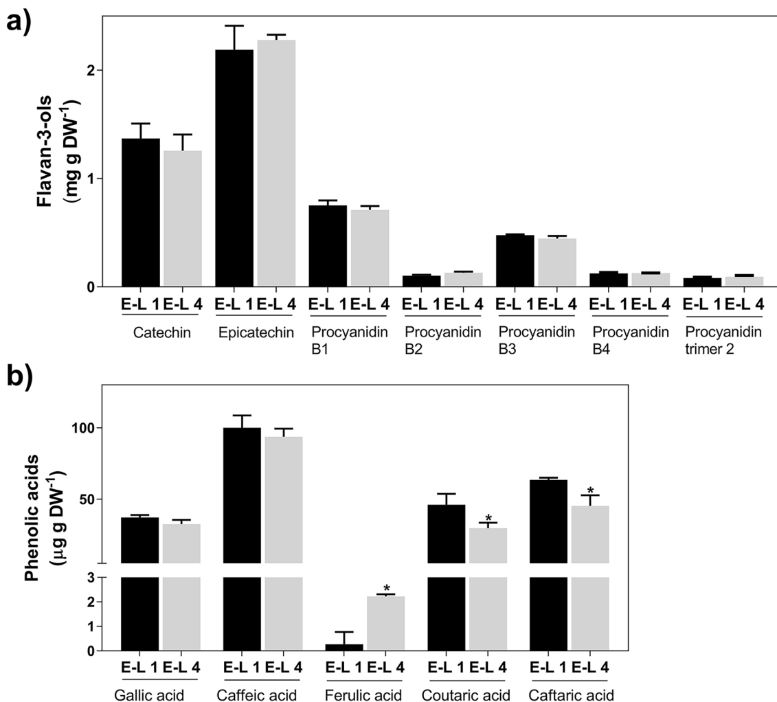
Fig. 4 Metabolomic analysis of flavan-3-ols ( a ) and phenolic acids ( b ) in grapevine canes at E-L 1 and E-L 4. Asterisks denote statistically significant differences between E-L 4 and E-L 1 (Mean values \pm SD, n = 3 , *P \leq 0.05 )
