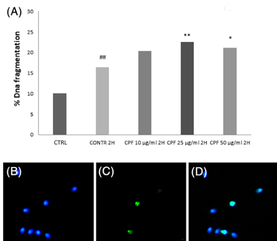
Fig. 3. Effects of different chlorpyrifos concentrations (10 \mu\text{g}/\text{mL} , 25 \mu\text{g}/\text{mL} , and 50 \mu\text{g}/\text{mL} ) on sperm DNA fragmentation (A). ###Highly significant differences relative to the control 0 hr ( P < 0.01 ); *,**Significant and highly significant compared to the corresponding control (1 hr and 2 hr) ( P < 0.05 ; P < 0.01 ). (B) Hoechst stained spermatozoa; (C) Tunnel positive spermatozoa; (D) Merge.
