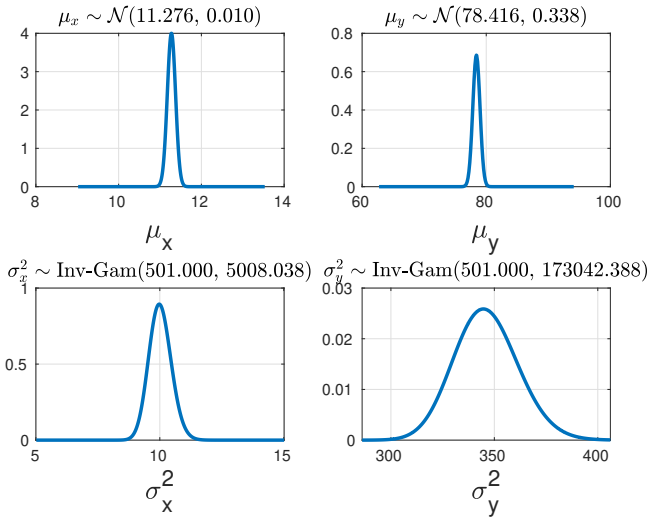
Fig. 3: Approximate marginal posterior density function for \mu_x , \sigma_x^2 , \mu_y and \sigma_y^2 estimated by MFVB.
