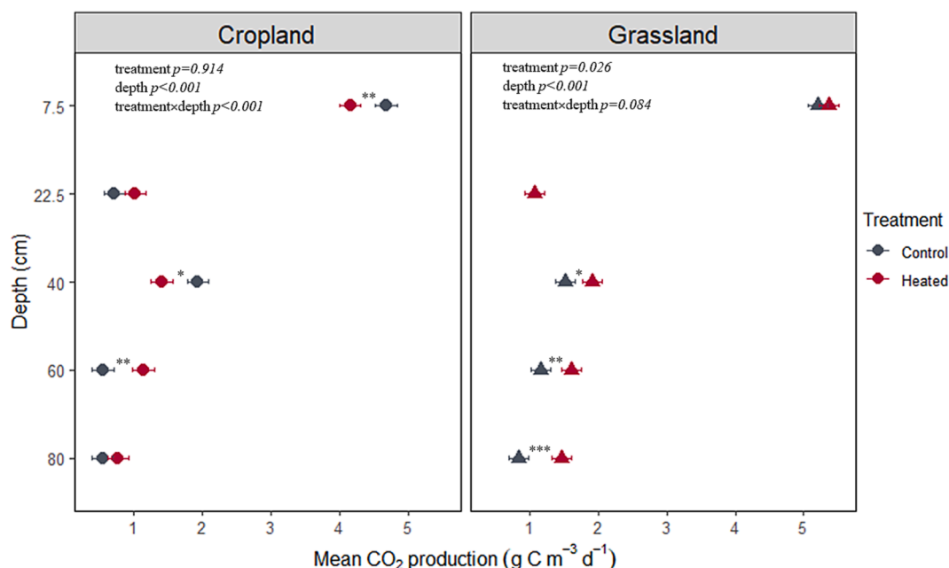
Fig. 6. Mean CO 2 production (g C m -3 d -1 ) in the control and heated plots (mean \pm SE, n = 3 ) with depth increment (0–15, 15–30, 30–50, 50–70, and 70–90 cm) over the study period (January 2022 to June 2022). In the figure, the p -values denote the statistically significant effects of treatment, depth, and their interaction (treatment \times depth). The asterisk indicates any significant treatment effect within depth as determined by post hoc analysis (* p \leq 0.05 ; ** p \leq 0.01 ; *** p \leq 0.001 ).
