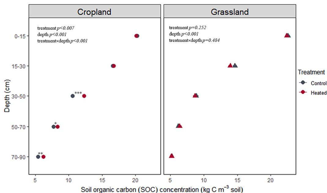
Fig. 7. Soil organic carbon (SOC) concentration (kg C m -3 soil) in the control and heated plots (mean \pm SE, n = 3 ) with depth increment (0–15, 15–30, 30–50, 50–70, and 70–90 cm), sampled in May 2022, one year after the onset of in-situ warming. In the figure, the p -values denote the statistically significant effects of treatment, depth, and their interaction (treatment \times depth). The asterisk indicates any significant treatment effect within depth as determined by post hoc analysis (* p \leq 0.05 ; ** p \leq 0.01 ; *** p \leq 0.001 ).
