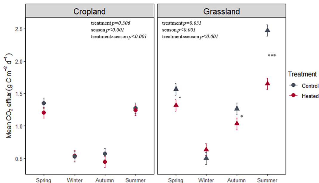
Fig. 5. Mean seasonal variations of soil \text{CO}_2 efflux ( \text{g C m}^{-2} \text{d}^{-1} ) in the control and heated plots (mean \pm SE, n = 3 ) from the whole-soil profile over the study period (July 2021 to June 2022). In the figure, the p -values denote the statistically significant effects of treatment, season, and their interaction (treatment \times season). The asterisk indicates any significant treatment effect within season as determined by post hoc analysis (* p \leq 0.05 ; ** p \leq 0.01 ; *** p \leq 0.001 ).
