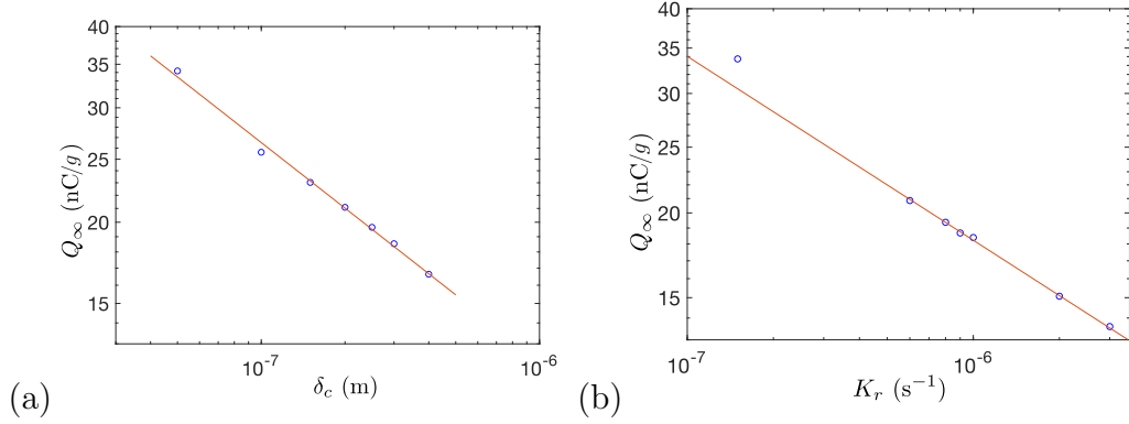
Figure 9: (a) Saturation charge as a function of tunneling distance from numerical simulations and its power-law fit Q_\infty = 1.038 \cdot 10^{-10} \delta_c^{-0.335} ; (b) Saturation charge as a function of the relaxation parameter K_r from numerical simulations and its power-law fit Q_\infty = 4.31 \cdot 10^{-10} K_r^{-0.271} .
