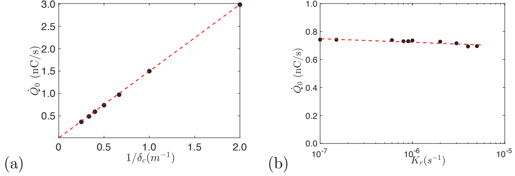
Figure 8: Charging rate for a granular bed of mass of 1 g (a) as a function of the inverse of tunneling distance 1/\delta_c with K_r = 10^{-6} s^{-1} and its linear approximation \dot{Q}_0 = 1.50 \cdot 10^{-7}/\delta_c ; (b) as a function of the relaxation parameter K_r for \delta_c = 2 \cdot 10^{-7} m with its linear fit \dot{Q}_0 = -1.36 K_r + 0.75 nC/s.
