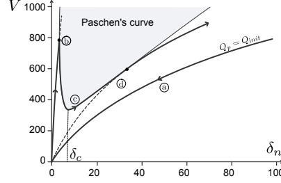
Figure 1: Paschen's limit curve describing the electric potential V necessary to initiate charge relaxation as a function of the gap \delta_n . The bold line illustrates variation of electric potential for a pair of particles before (a) and after (b–d) the creation of mechanical contact leading to a variation of charge. The dashed line represents the variation of electric potential after charge relaxation.
