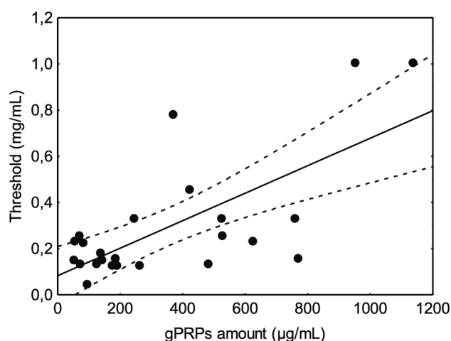
Fig. 6. Spearman correlation between astringency threshold and the mean gPRPs observed in the group of young panellists. The solid line corresponds to the fitted data. The dotted line corresponds to the confidence interval at 95%. The black dots represent individual data points.
