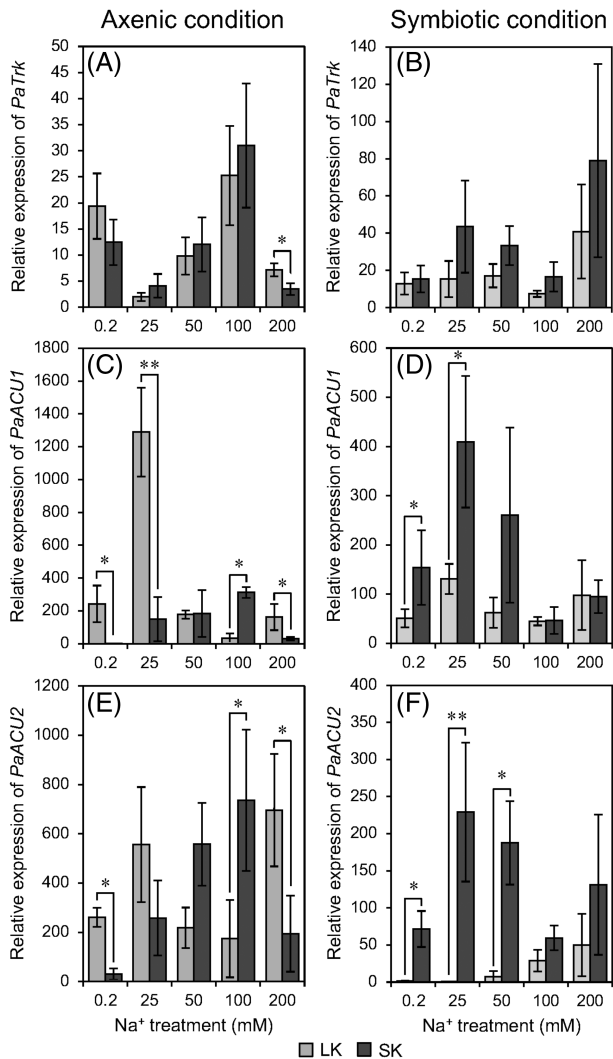
FIGURE 3 Relative expression of putative K + transporters in Paxillus ammoniaevirescens grown in axenic or symbiotic conditions with limited or sufficient potassium availability at varying levels of sodium exposure. Relative expressions of the putative K + transporters PaTrk (A), PaACU1 (C), and PaACU2 (E) were determined by RT-qPCR in thalli grown in liquid media with 0.05 mM (LK) or 1.0 mM (SK) of potassium (K + ) and exposed for 3 weeks to either 0.2, 25, 50, 100, or 200 mM of sodium (Na + ). PaTrk (B), PaACU1 (D), and PaACU2 (F) expression levels were also determined by RT-qPCR in P. taeda roots colonized by P. ammoniaevirescens (Pa) for eight weeks, in either LK or SK conditions, and exposed for 4 weeks to the same Na + treatments. The results are based on two to four biological replicates and three technical replicates. Statistical differences between LK and SK conditions for each Na + treatment point were determined using the Student's test. P < 0.05 (*) and P < 0.01 (**).
