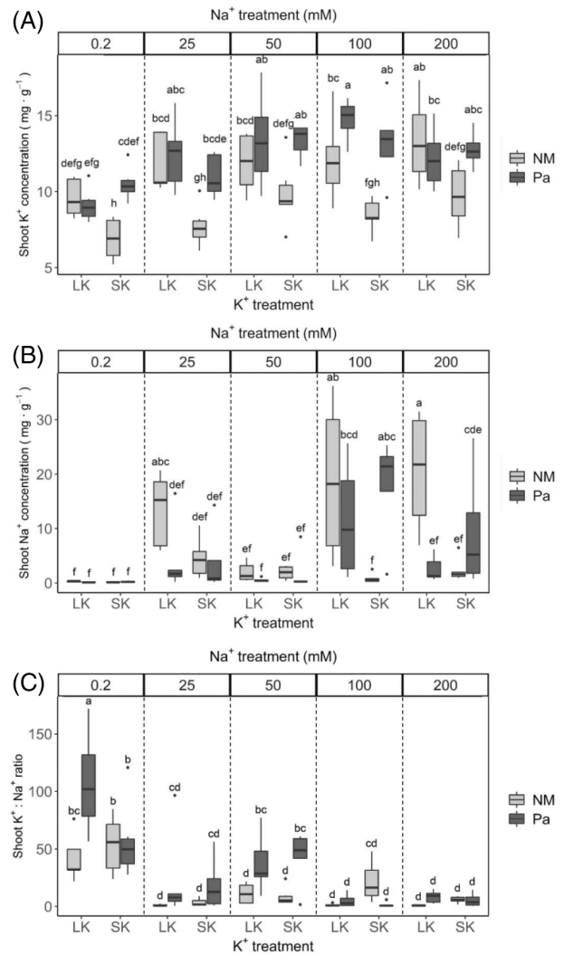
FIGURE 6 Shoot potassium and sodium concentrations and ratios in Pinus taeda seedlings, inoculated or not with Paxillus ammoniaevirescens and grown with limited or sufficient potassium availability at varying levels of sodium exposure. Potassium (K + , A) and sodium (Na + , B) concentrations were determined by ICP-OES, in the shoot of P. taeda seedlings 8 weeks after inoculation with P. ammoniaevirescens (Pa) or not (NM) in either 0.05 mM (LK) or 1.0 mM (SK) of K + , and exposed for 4 weeks to either 0.2, 25, 50, 100, or 200 mM of Na + . (C) Ratios between shoot K + and Na + concentrations were calculated for each pine seedling. Median values are indicated by horizontal lines within boxplots, and whiskers on top and bottom extend from the first quartile to minimum and from the third quartile to maximum values, respectively. Different letters above boxplots indicate significant differences between treatments according to 3-way ANOVA followed by LSD post hoc test at P ≤ 0.05. n = 4–6.
