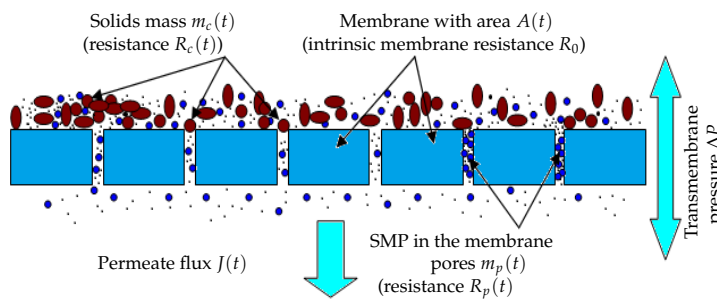
Figure 1. Membrane fouling by cake formation and pores clogging.
