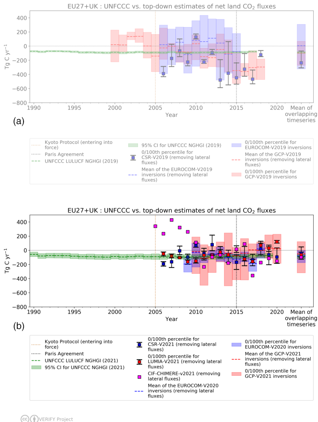
Figure B5. Comparison of inventories and atmospheric inversions for the total EU27+UK biogenic CO 2 fluxes from Petrescu et al. (2021) (a) and updated data from current study (b). Top-down inversion results are the following: the global GCB2021 ensemble, the regional EUROCOM ensemble, the regional CarboScopeReg model with multiple variants, the regional LUMIA model with multiple variants, and CIF-CHIMERE. The relative error in the UNFCCC values represents the UNFCCC NGHGI (2021) member states reported uncertainty computed with the error propagation method (95 % confidence interval) gap-filled and provided for every year of the time series. The time series mean overlapping period is 2010–2018. The colored area represents the min/max of model ensemble estimates. The same emissions due to lateral fluxes of carbon through rivers, crop trade, and wood trade are removed from the top-down estimates in both the top and bottom graphs for consistency. The fluxes follow the atmospheric convention, where negative values represent a sink, while positive values represent a source. Note that Petrescu et al. (2021) presented the top plot including a suite of bottom-up models, which have been removed here for clarity.
