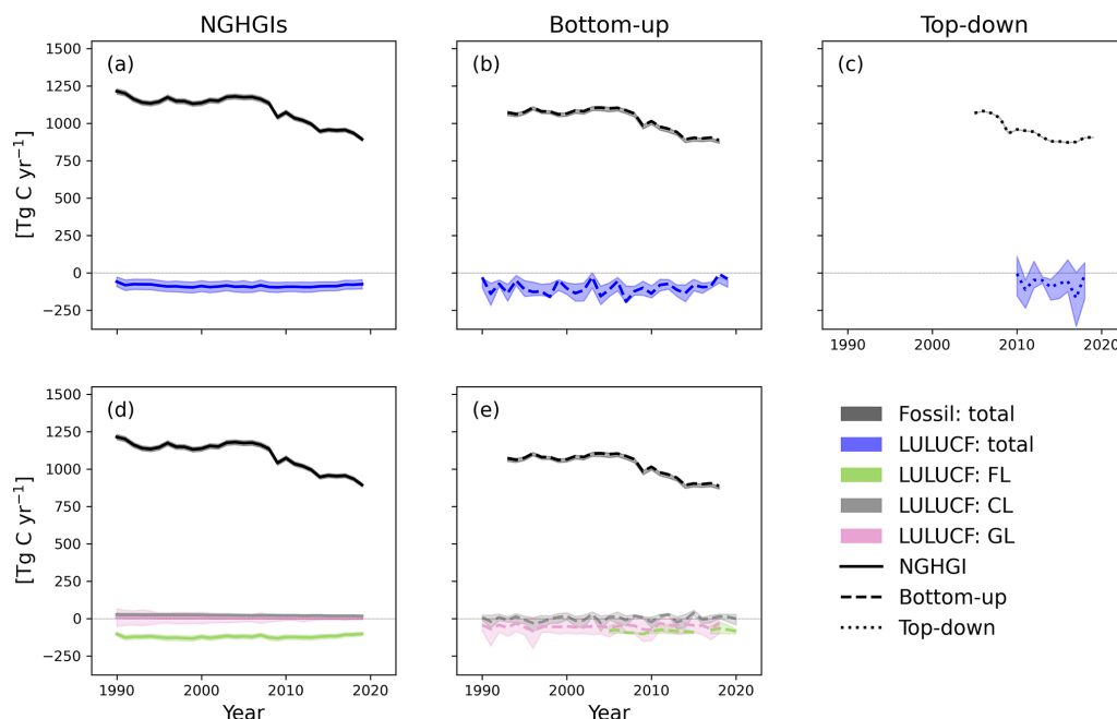
Figure 1. A synthesis of all the CO 2 net fluxes shown in this work for the EU27+UK. The estimates are divided by approach: NGHGI estimates (a, d), bottom-up methods (b, e), and top-down methods (c). Panels (d) and (e) include a breakdown of the (bottom-up) LULUCF flux into three of the dominant components: FL, GL, and CL. Such a breakdown is not provided for NGHGI CO 2 fossil as partitioning of bottom-up CO 2 fossil datasets corresponding to UNFCCC NGHGI categories is not currently available. The NGHGI UNFCCC uncertainty is calculated for submission year 2021 as the relative error of the NGHGI value, computed with the 95 % confidence interval method gap-filled and provided for every year of the time series, except for FL, GL, and CL, which are taken directly from the EU NIR (2021). Shaded areas for the other estimates represent the 0th–100th percentiles for groups with fewer than seven members and the 25th–75th percentile for groups with seven or more members. Ensembles (e.g., TRENDY v10) are included in the above only for their mean values to avoid more heavily weighting the ensembles compared to the other datasets.
