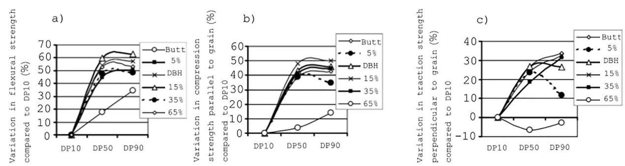
Fig. 20 Variation of a flexural strength, b compression strength parallel to grain, and c traction strength perpendicular to grain relative to properties measured at 10% of total radius DP10 as a function of radius from the pith and percentage of total height for Pinus Pinaster Ait., adapted from [146]
