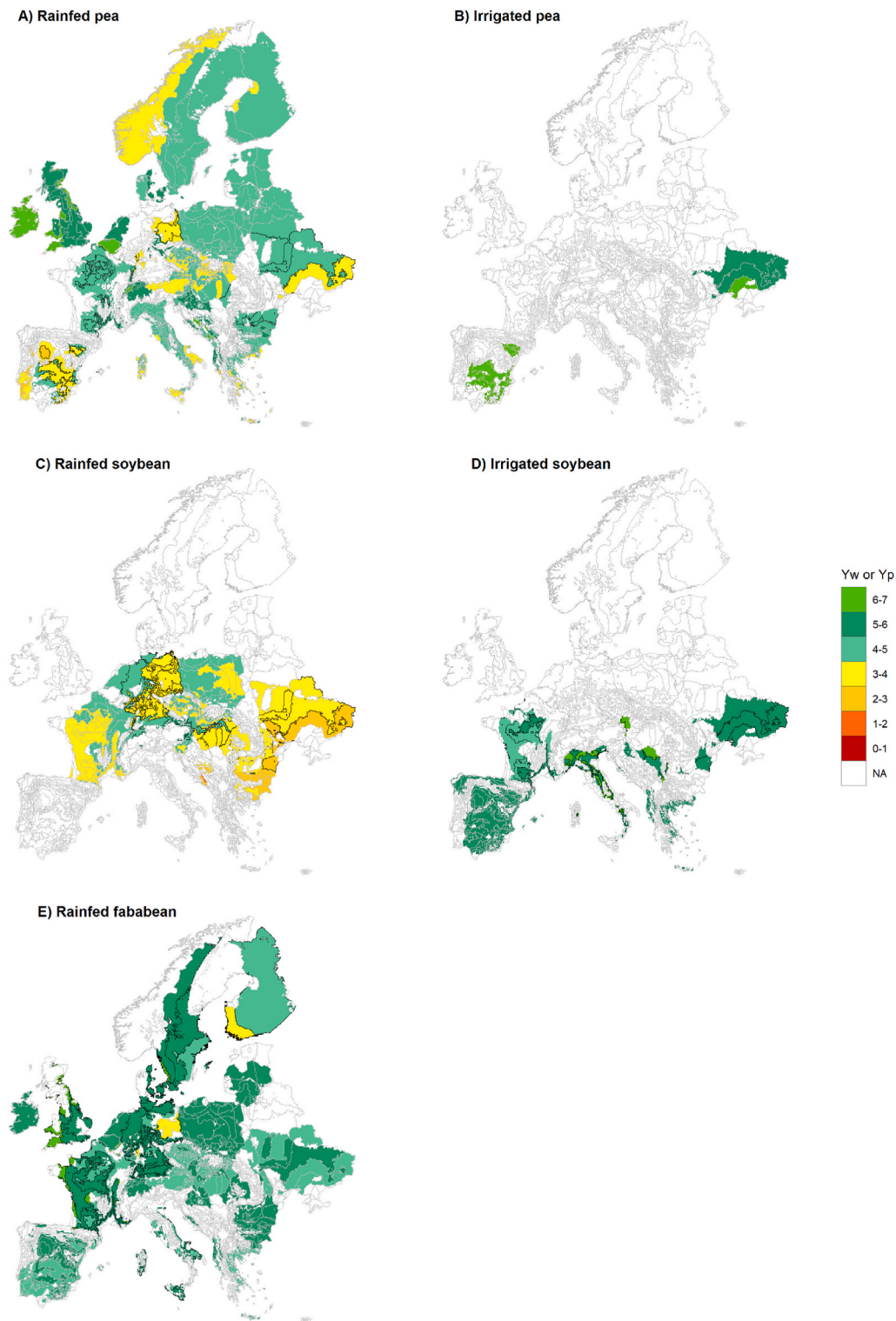
Fig. 1. Water limited potential yield (Yw; left panels) and potential yield (Yp; right panels) in Mg ha -1 of pea (top panels), soybean (middle panels), faba bean (bottom panel) at climate zone level (note, Yw and Yp are presented for the whole climate zone but cultivation does not take place everywhere in that climate zone [e.g., no crop growth in the very north of Europe]). Black line around a climate zone means that data is estimated through crop growth simulation models (Method 1), while a grey line indicates results from the regression model (Method 2).
