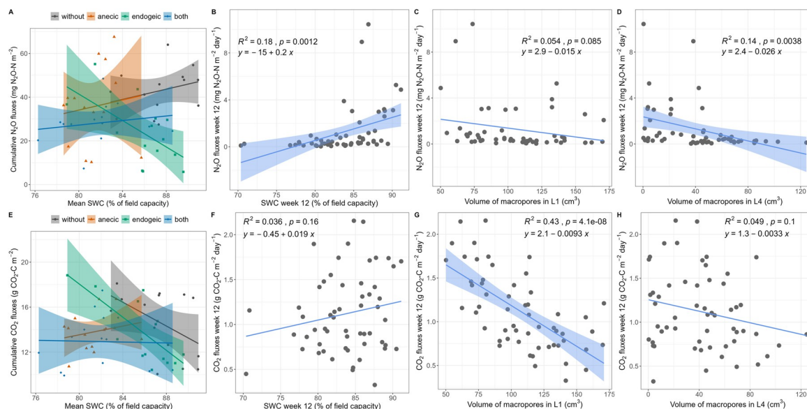
Fig 4. \text{N}_2\text{O} and \text{CO}_2 emissions as affected by soil water content and macroporosity. (A, E) Total cumulative emissions as affected by the Ew \times SWC interaction, where SWC represents the 3-month average SWC. (B, C, D, F, G, H) Relationships between \text{N}_2\text{O} and \text{CO}_2 emissions measured in the last experimental week (week 12), (C, F) soil water contents and (D, G) X-ray tomography estimated volumes of macropores in the topsoil layer (L1) and (D, H) in the bottom layer for \text{N}_2\text{O} (L4). When significant, the linear regression line and 95% confidence intervals are displayed along with the regression equation, coefficient of determination ( R^2 ) and p value. Note that this relationship may differ from the mixed-effect model results (Tables 1 and 4).
