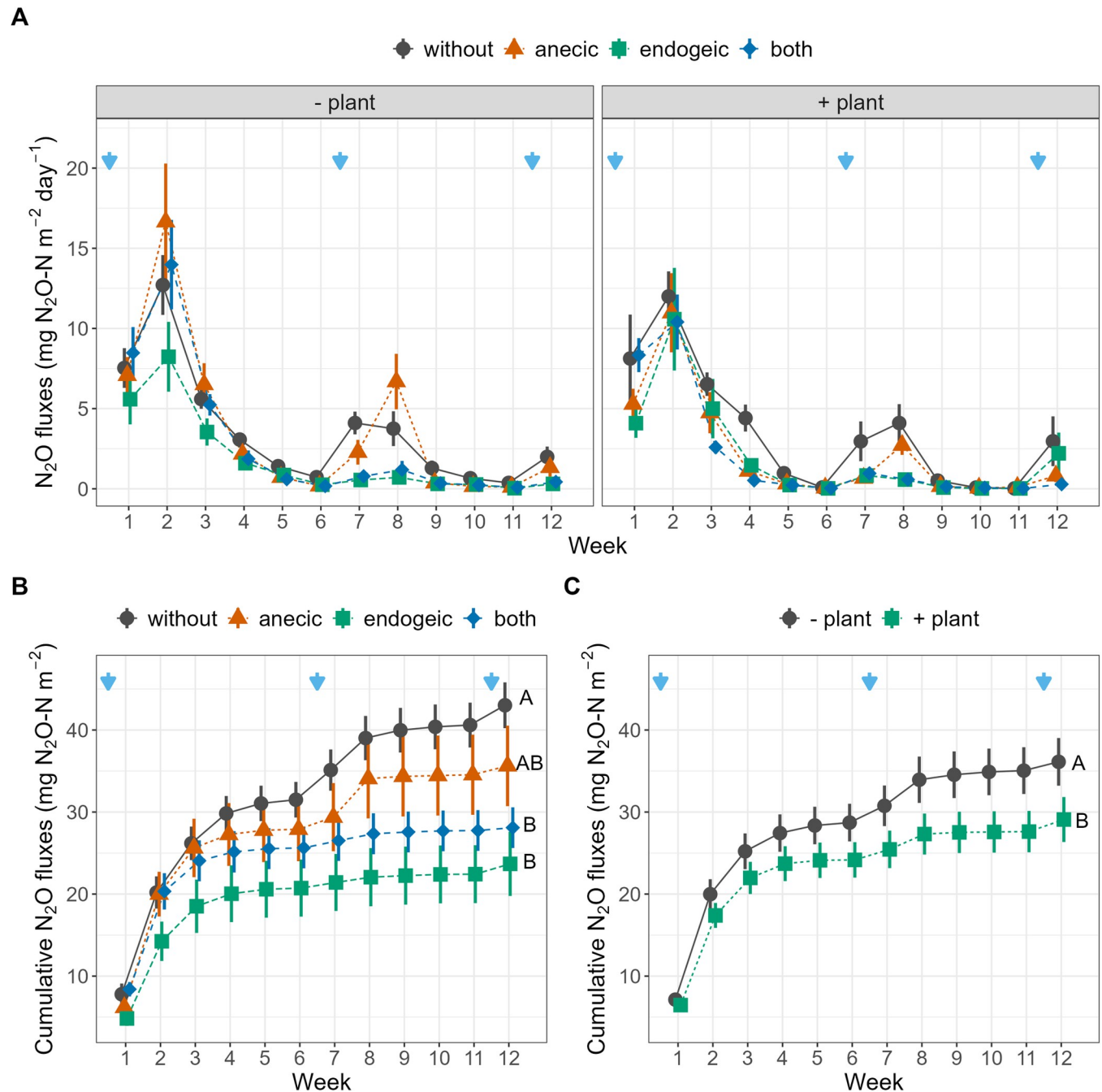
Fig 2. \text{N}_2\text{O} emissions during the 12-week experiment. (A) Weekly (B, C) and cumulative \text{N}-\text{N}_2\text{O} emissions as affected by the earthworm and plant treatments. Blue arrows represent watering events. Error bars represent \pm 1 SEM. Different letters represent significantly different levels as estimated by Tukey's HSD post hoc test. The effects of earthworm treatment independent of plant treatment, and vice-versa, are displayed when the \text{Ew} \times \text{Plant} interaction is not significant (B, C).
