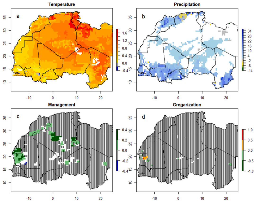
Fig. 4. Comparison of trend maps at 0.5° cells. The study area was divided in 0.5° grid cells. Only cells with significant temporal trends are colored: a-trend of annual mean temperatures (°C of increase/decrease) and b-trend of annual mean precipitations (mm of increase/decrease), which were both determined with the harmonic seasonal model; c- Trend of the number of pesticide applications each year (number per year). Vertical stripes indicate cells that were visited less than three times over the study period (had less than three years with management operations); d- Annual trend of the number of observation points with gregarious hoppers on total surveys (number per year). The vertical stripes on the area hide cells with less than three observations of gregarious occurrences.
