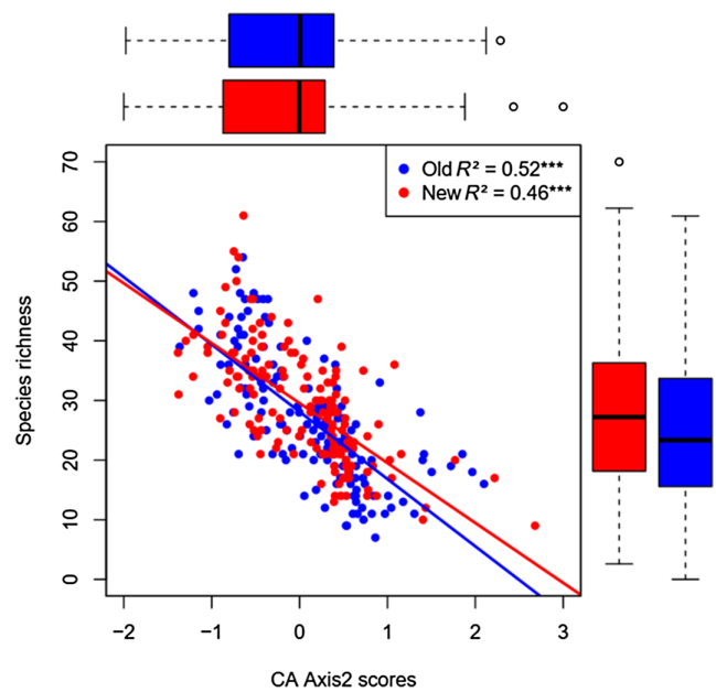
FIGURE 6 Changes in species richness with increasing plot scores on axis 2 (related to decreasing irradiance) of the correspondence analysis conducted on the vegetation composition of the 314 plots of the Sancy site (1988–1989 plots and curve are in blue and 2022 ones in red). Regression coefficients and significances of the linear curves are indicated on the top right of the graph (***, p < 0.001 ).
