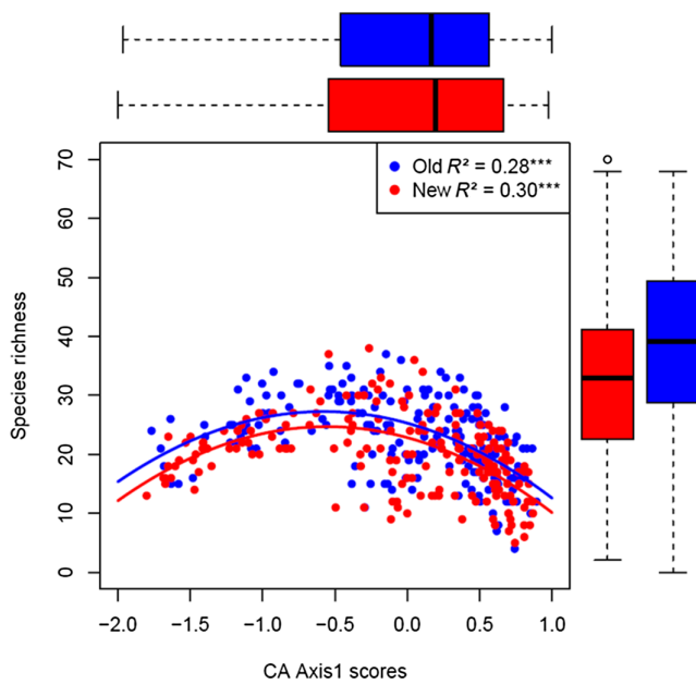
FIGURE 4 Changes in species richness with increasing plot scores on axis 1 (related to increasing vegetation biomass) of the correspondence analysis conducted on the vegetation composition of the 378 plots of the Alpe d'Huez site (1997 plots and curve are in blue and 2017–2018 ones in red). Regression coefficients and significances of the polynomial curves are indicated on the top right of the graph (***, p < 0.001 ).
