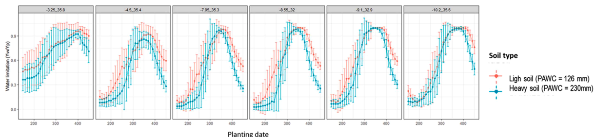
Fig. 2. Average simulated (20 years, model ensemble only) ratio of water-limited yield to potential yield ( Y_w/Y_p ) for six locations (the title of the panel gives the latitude and longitude) and 31 sowing dates in Tanzania. Vertical bars are standard deviations attributed to the different simulated years. Model simulations start 150 days before planting so that the first planting date is on the day of the year 150. The locations are in the southern hemisphere with a rainy season expanding from one year to the following one. Sowing dates are expressed in the number of days since January 1st of the first year of the rainy season. The last planting date has a value of 450 which correspond to model initialisation on the day of the year 300 and a planting date on day 85 of the second year of the season when the first year is not a leap year.
