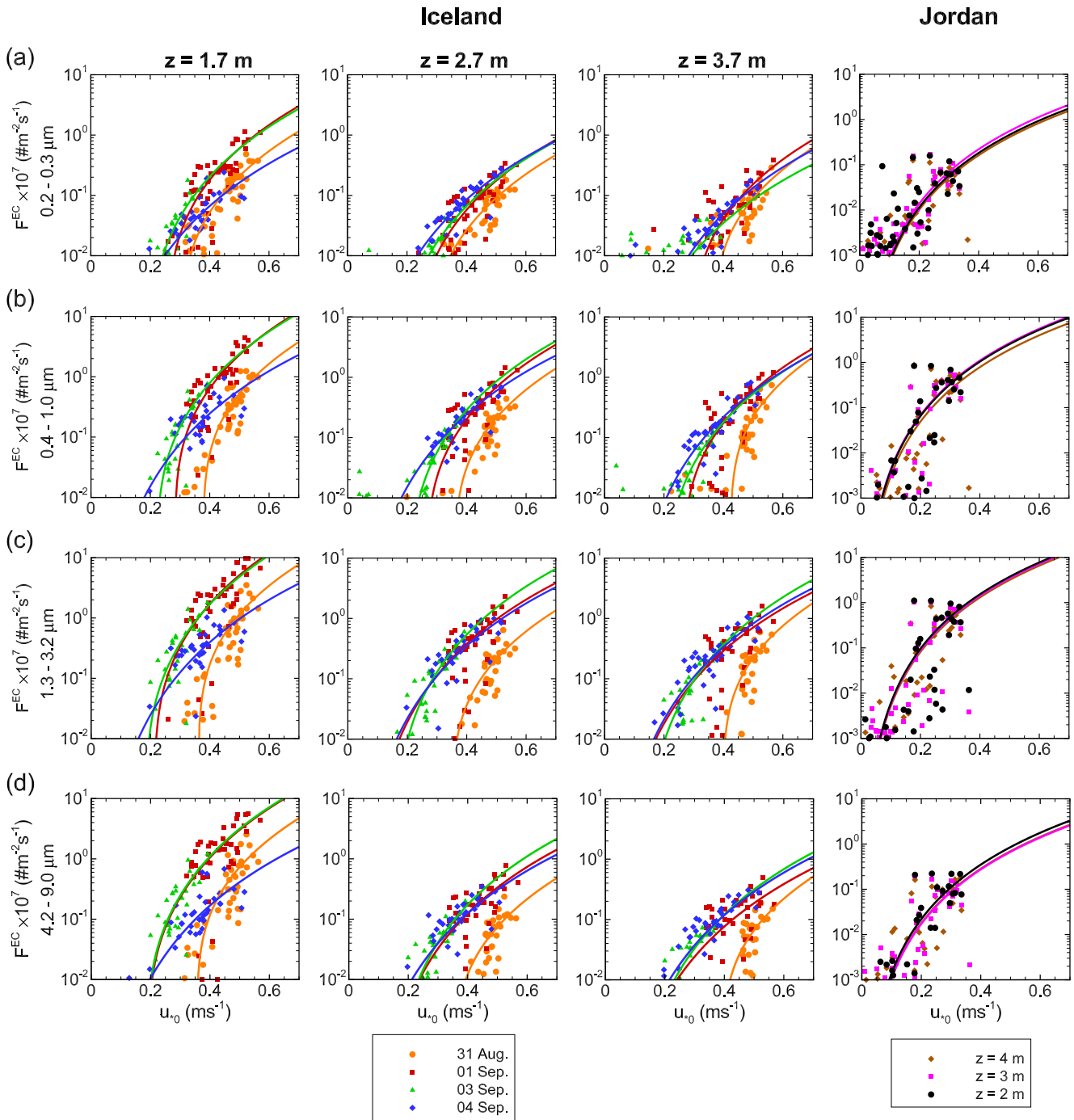
Figure 11. Dust fluxes F^{EC} as a function of the surface friction velocity u_{*0} for all erosion events in Iceland and in Jordan (right figures) and at the three measurement heights. Dust fluxes are in number and for four particle size ranges: 0.2–0.3 \mu\text{m} (a), 0.4–1.0 \mu\text{m} (b), 1.3–3.2 \mu\text{m} (c), and 4.2–9.0 \mu\text{m} (d). The solid curves are fit over each event and each height such as F^{EC} = au_{*0}^3(u_{*0} - \beta) . The color of these curves corresponds to the color of the associated dots.
