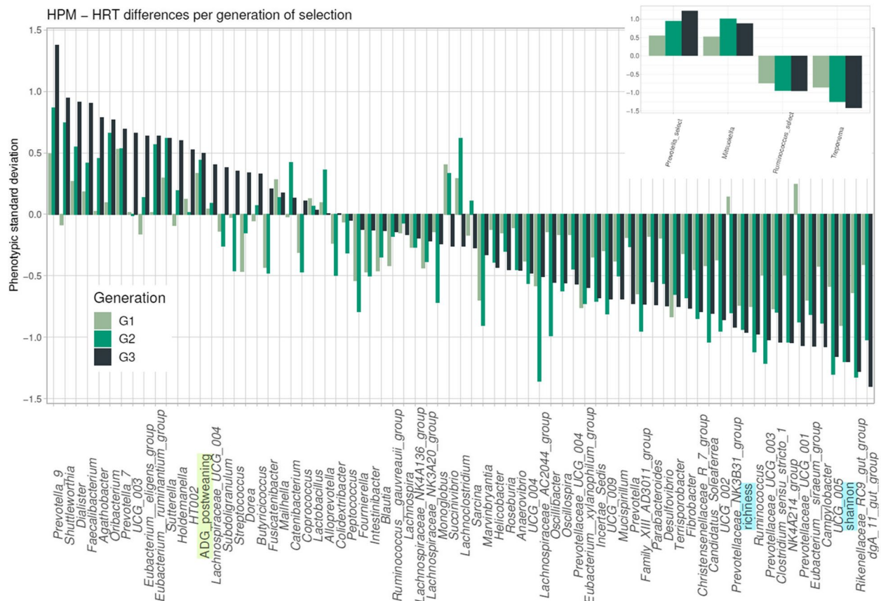
Fig. 4 Responses to genetic selection oriented towards a high abundance of Prevotella and Mitsuokella or a high abundance of Ruminococcus and Treponema at D60 across three generations. The differences between the HPM and HRT lines for 74 genera, 2 diversity indexes (light blue highlighting), and one growth feature (ADG_postweaning: average daily gain during the post-weaning period, light green highlighting) are expressed in standard deviation. They are ranked from the largest positive difference (on the left) to the largest negative difference (on the right) at generation G3 of the selection. The differences are in pale green for G1, green for G2, and dark green for G3. Positive differences are associated with higher values in the HPM line whereas negative values are associated with higher values in the HRT line. Microbiota results are based on 16S rRNA sequencing data
