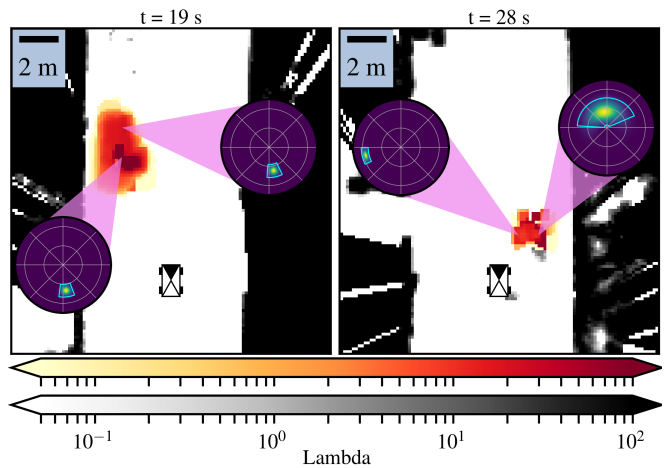
Fig. 6. Example of field resulting from our method, where the robot is located at the bottom center of the map. The static (resp. dynamic) environment is represented using a gray (resp. red) scale. A car is approaching the robot at t = 19 s, whereas a pedestrian is crossing the road at t = 28 s right in front of the robot. Some speed distributions of the cells are displayed in polar plots (angle for the orientation, radius for the velocity), where inner circles correspond to a step of 1 \text{ m s}^{-1} .
