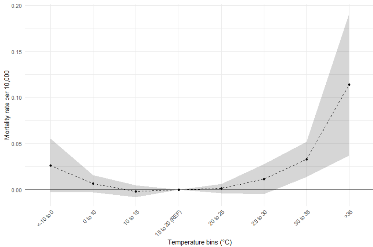
Figure 14: Coefficients of maximum temperature on mortality
