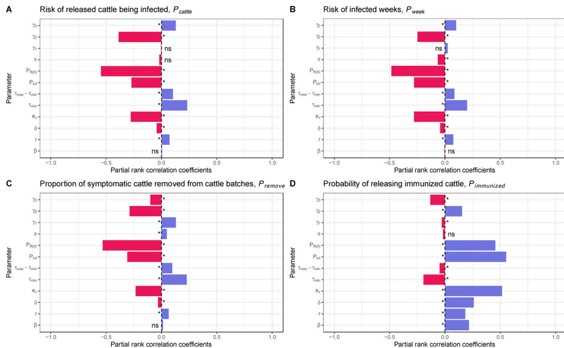
Fig. 6. Tornado plots of the partial rank correlation coefficients (PRCC) between the rank-transformed model parameters and rank-transformed risk estimates: A) The risk of released cattle being infected, P_{cattle} ; B) The risk of infected weeks, P_{week} ; C) The proportion of symptomatic cattle removed from cattle batches, P_{remove} ; D) Probability of releasing immunized cattle, P_{immunized} . Asterisks (*) indicate that the PRCC statistics are significantly different from 0 ( p < 0.05 ), while “ns” indicates the non-significant PRCC statistics. Model parameters shown in the X-axis were following (from bottom to top): 1) Within-herd transmission coefficient, \beta ; 2) The reduction factor of between-batch transmission, r ; 3) The proportional infectiousness of asymptomatic individuals, \delta ; 4) Vaccine effectiveness, e_v ; 5) Minimum time-to-immunity, \tau_{\min} ; 6) Difference between maximum and minimum time-to-immunity, \tau_{\max} - \tau_{\min} ; 6) Probability of imported cattle being FMDV infected, P_{inf} ; 7) Proportion of non-infected newly imported cattle having immunity at arrival, P_{R(0)} ; 8) Proportion of infectious individuals becoming symptomatic, \pi ; 9) Recovery rate of asymptomatic individuals, \gamma_1 ; 10) Transition rate from asymptomatic to symptomatic individuals, \gamma_2 ; 11) Recovery rate of symptomatic individuals, \gamma_3 .
