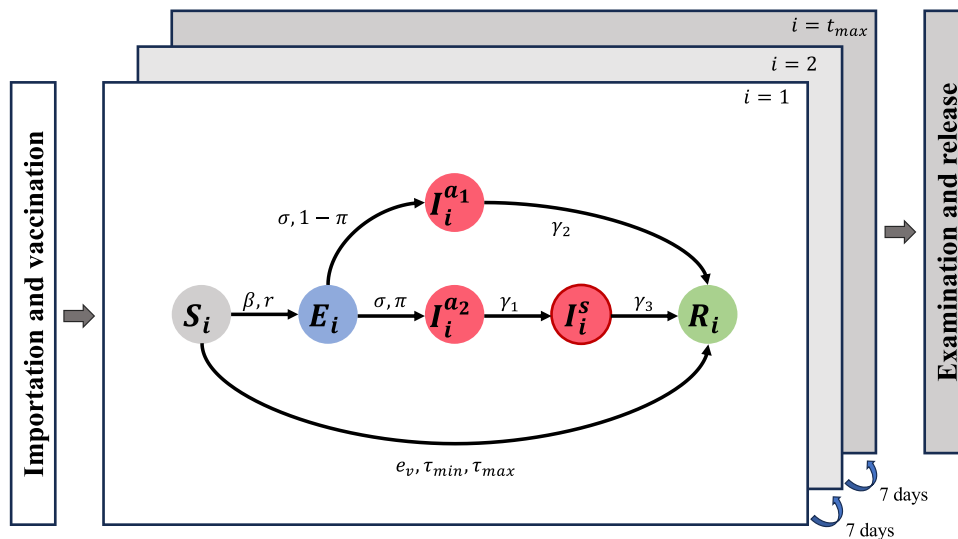
Fig. 2. A conceptual framework for disease dynamics model. Cattle are classified according to the epidemiological statuses as susceptible ( S ), exposed ( E ), asymptomatic infectious ( I^{a1} and I^{a2} ), symptomatic infectious ( I^s ), and recovered ( R ). New cattle are imported across the border into the quarantine center every seven days. FMDV transmission could occur among the cattle from different batch-weeks i \in \{1, 2, \dots, t_{max}\} . Cattle are examined and released once they stay quarantined for t_{max} weeks. The compartment transition processes were mathematically described in Eqs. (1)–(17). Parameters indicated in the diagram included 1) Within-herd transmission coefficient, \beta ; 2) The reduction factor of between-batch transmission, r ; 3) The proportional infectiousness of asymptomatic individuals, \delta ; 4) Vaccine effectiveness, e_v ; 5) Minimum time-to-immunity, \tau_{min} ; 6) Maximum time-to-immunity, \tau_{max} ; 7) Proportion of infectious individuals becoming asymptomatic, \pi ; 8) Recovery rate of asymptomatic individuals, \gamma_1 ; 9) Transition rate from asymptomatic to symptomatic individuals, \gamma_2 ; 10) Recovery rate of symptomatic individuals, \gamma_3 .
