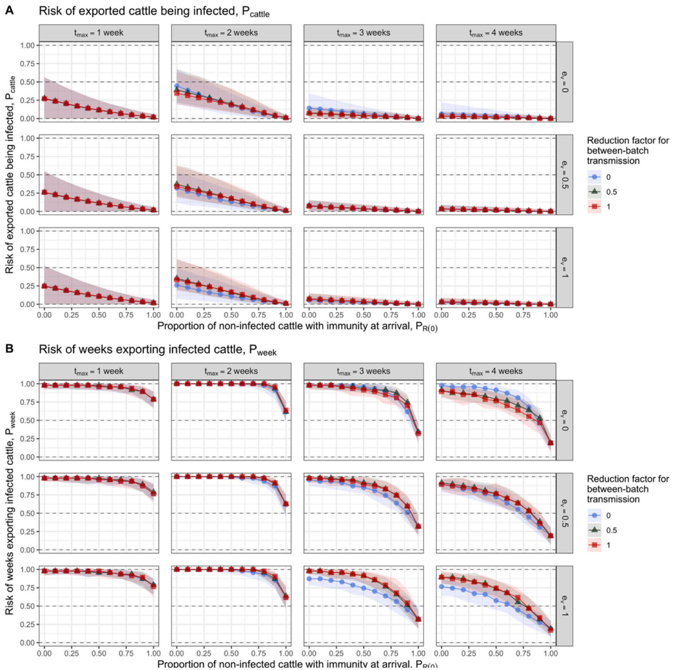
Fig. 4. Risks of releasing infected cattle to the market per batch; A) Risk of released cattle being infected, P_{cattle} ; B) Risk of infected weeks, P_{week} . Risk estimates on the Y-axis were evaluated across various combinations of the following model parameters: 1) The proportion of non-infected cattle with immunity at arrival, P_{R(0)} , displayed on the X-axis; 2) The reduction factor of the between-batch transmission, r . Colors and shapes indicate different levels of the reduction factor: r = 0 , no between-batch transmission (dark blue circle); r = 0.5 , the between-batch transmission is reduced by 50 % (green triangle); r = 1 , no reduction on the between-batch transmission (red square); 3) Vaccine effectiveness, e_v , of 0.0, 0.5, and 1.0; 4) Quarantine period, t_{max} of 1, 2, 3, and 4 week(s). Risk estimates shown in this figure were the median (symbols) and the 95 % CI (shaded areas) across 100 iterations.
