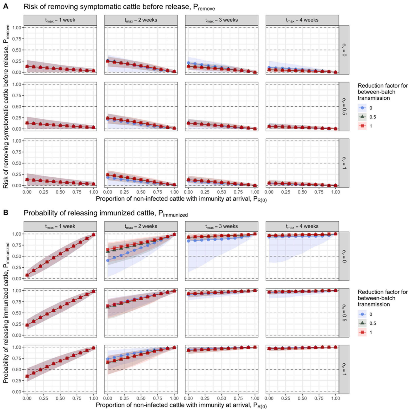
Fig. 5. Risks of releasing infected cattle to the market per batch; A) Risk of symptomatic cattle removed from the cattle batch, P_{remove} ; B) Probability of releasing immunized cattle, P_{immunized} . Risk estimates on the Y-axis were evaluated across various combinations of the following model parameters: 1) The proportion of non-infected cattle with immunity at arrival, P_{R(0)} , displayed on the X-axis; 2) The reduction factor of the between-batch transmission, r . Colors and shapes indicate different levels of the reduction factor: r = 0 , no between-batch transmission (dark blue circle); r = 0.5 , the between-batch transmission is reduced by 50 % (green triangle); r = 1 , no reduction on the between-batch transmission (red square); 3) Vaccine effectiveness, e_v of 0.0, 0.5, and 1.0; 4) Quarantine period, t_{max} of 1, 2, 3, and 4 week(s). Risk estimates shown in this figure were the median (symbols) and the 95 % CI (shaded areas) across 100 iterations.
