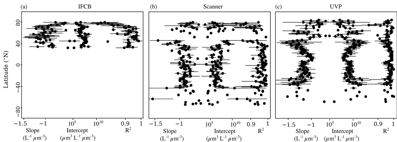
Figure 5. Latitudinal variability of NBSS slopes, intercepts, and determination coefficients for the IFCB (a), scanners (b), and the UVP (c). Dots represent the mean parameter value per 1^{\circ} latitudinal bins, and the horizontal bars represent the standard deviation.
