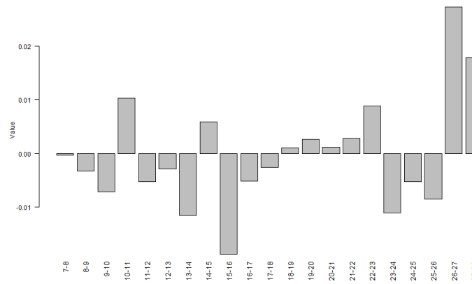
Fig. 11 Estimated clr coefficients of tmin in the discrete regression
