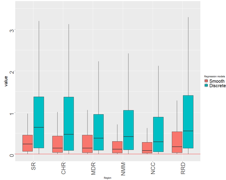
Fig. 9 Distance between observed and fitted values by models and regions
