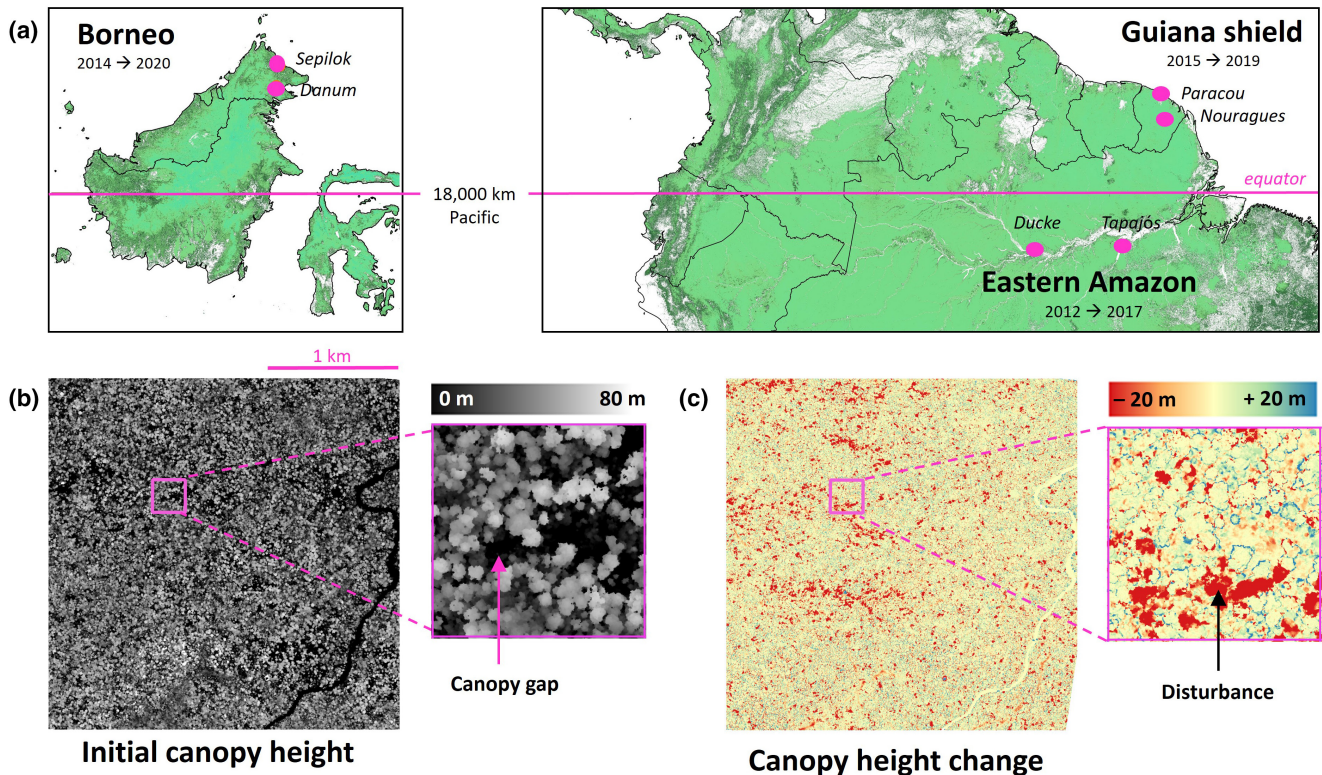
FIGURE 1 A map of the study sites and an example of the repeat LiDAR data used in this study. (a) Map of study sites overlaid onto forest cover map (green=forest and white=non-forest) derived from Global Ecosystems Dynamics Investigation data. (b) Example of canopy height rasters derived from LiDAR data from Danum, Malaysia. Smaller panels show a close-up of a 10-ha forest patch. (c) Canopy height change rasters for the same area as in (b). Map lines delineate study areas and do not necessarily depict accepted national boundaries.
