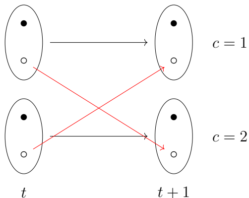
Figure 10: General representation of the interacting PO-DBN with interactions between hidden life stages of the C = 2 populations. An empty circle represents a hidden life stage and a filled one is an observed life stage.
