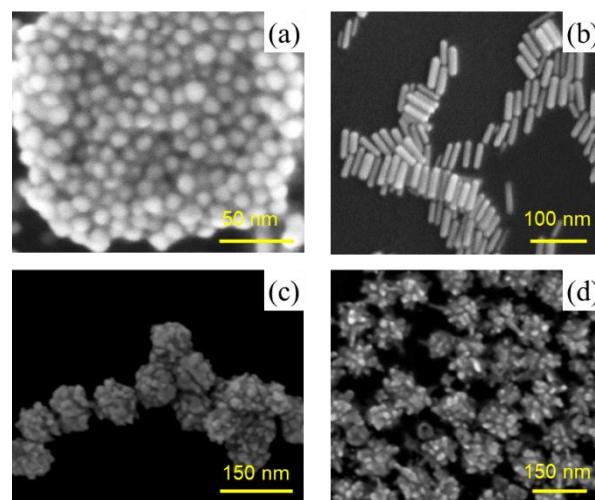
Figure 1. SEM images of (a) AuNSP-citrate, (b) AuNRO-CTAB, (c) AuNFL-dopamine and (d) AuNST-PVP.
