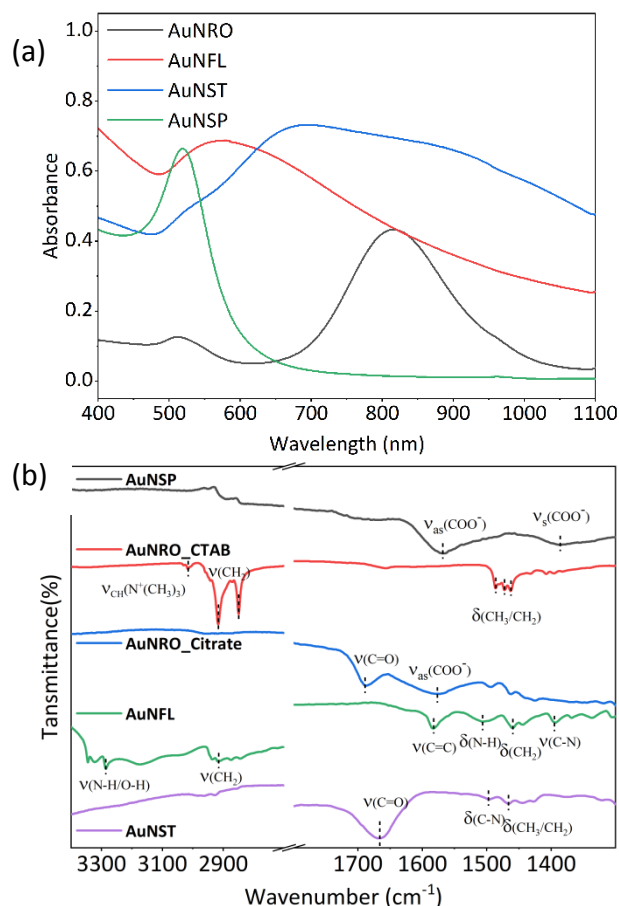
Figure 2. (a) Vis-NIR absorption spectra (400–1100 nm) of AuNSP-citrate, AuNRO-CTAB, AuNFL-dopamine, and AuNST-PVP, [Au 0 ] = 0.2 mM. (b) ATR-FTIR spectra of the same.
