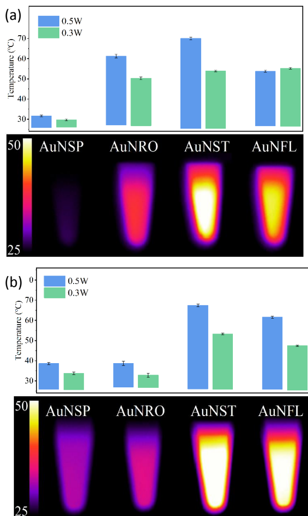
Figure 3. Plateau temperatures reached after 5 min. of irradiation at 808 nm (a) or 1064 nm (b) of AuNP suspensions: AuNSP-citrate, AuNRO-citrate, AuNFL-dopamine, and AuNST-PVP, [Au^0] = 0.2 mM.
