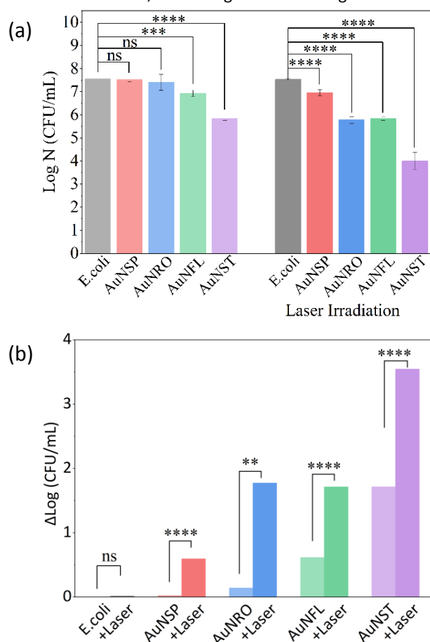
Figure 4. (a) \log N(\text{CFU/mL}) and (b) \Delta \log N(\text{CFU/mL}) of E. coli in the stationary phase, after incubation with different AuNP suspensions (AuNSP-citrate, AuNRO-citrate, AuNFL-dopamine, and AuNST-PVP) followed or not by irradiation (808 nm, power: 0.5 W). All experiments were performed in triplicate; error bars indicate standard deviations. Significance: non-significant (ns) for P > 0.05 , * for P \leq 0.05 (significant), ** for P \leq 0.01 (highly), *** for P \leq 0.001 (very highly), and **** for P \leq 0.0001 (extremely).
