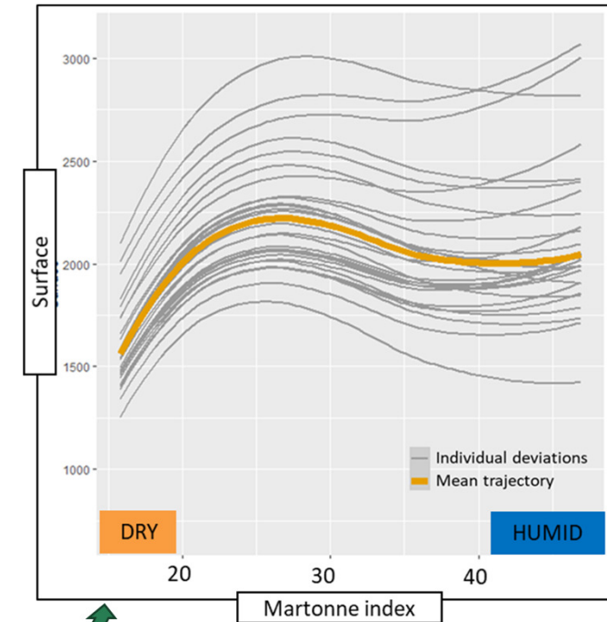
Ring surface modelisation by RR
