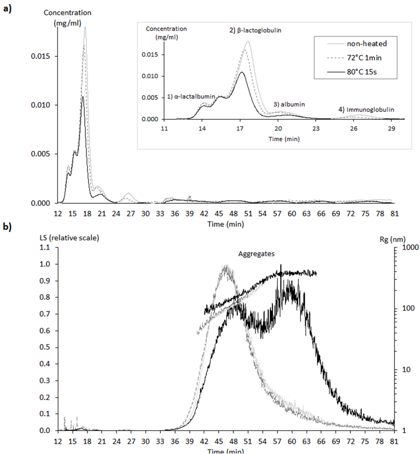
Fig. 4. (a) AF4 Fractogram of the protein concentrations (dRI signal) of raw and pasteurised sheep whey (72 °C/1 min and 80 °C/15 s) for the April period, with a magnification of the period between 11 and 29 min; (b) Fractogram of the MALS signal and radius of gyration (Rg) distribution of proteins in raw and pasteurised sheep whey (72 °C/1 min and 80 °C/15 s) for the April period.
