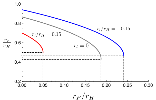
FIG. 5. Plot showing the contact radius as a function of force for different values of line tension: r_l = 0 (gray), r_l/r_H = 0.15 (red), and r_l/r_H = -0.15 (blue). For all the plots \theta_0 = \pi/6 . The dotted lines mark the contact radius and force at detachment.
