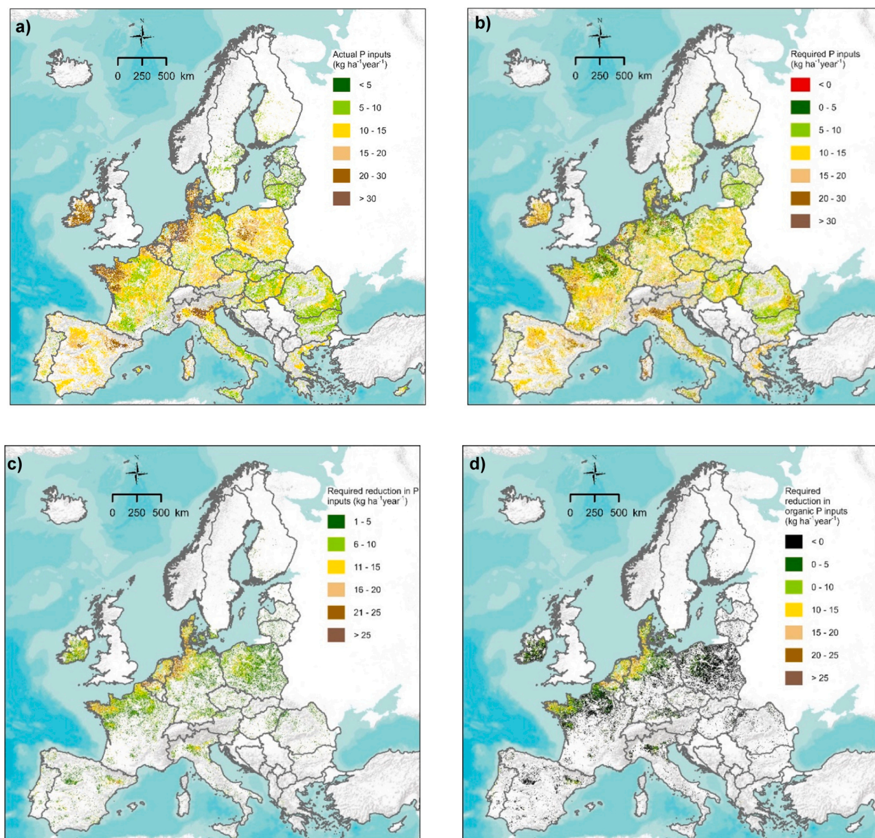
Fig. 3. (a) Actual inputs ( \text{kg ha}^{-1} \text{year}^{-1} ) taken from Muntwyler et al. (2024); (b) required P inputs ( \text{kg ha}^{-1} \text{year}^{-1} ) according to our calculations. The regions in red in Fig. b are those regions with high P_{\text{OLSEN}} concentrations, where according to our calculations, after 41 years with zero P inputs the P_{\text{OLSEN}} concentrations will still be higher than 40 \text{ mg kg}^{-1} ; (c) The reduction in P inputs needed to have the sustainable management practice in line with soil P concentrations and to reach optimal P concentrations in 41 years (solid arrows in Fig. 1); (d) The reduction of current organic P inputs needed to reach optimal P concentrations in 41 years. When zero reduction in P inputs are needed, it means that all the input reduction shown in Fig. 4a can be covered by reducing mineral P inputs.
