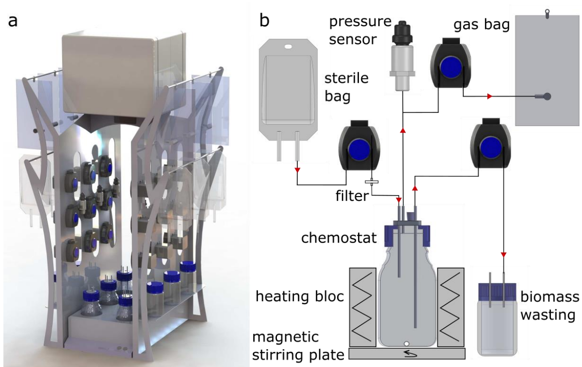
Figure 10 General view of the LAMACs and of components of one chemostat in the LAMACs module. a) 3D view of a LAMACs module, i.e., six chemostats. The electric box containing controlling cards is on the top of the module and above any source of liquids to prevent electric failure in case of leakage. A waterproof stirring plate is underneath the heating block containing the six reactor vessels. Three peristaltic pumps are aligned above each vessel. The upper range of bags is for biogas collection; the lower range serves as substrate reservoirs. The dimensions of one module are 50 cm width \times 52 cm length \times 100 cm height. b) Schematic view of a chemostat detailing the use of the three-hose connector. One port is used as inlet for feeding, and two ports as outlet for biomass wasting and degassing. One port for manual sampling is sealed with a rubber stopper. A 0.45 \mu\text{m} pore-size filter is placed in the feedline ahead of the reactor to prevent contamination of the medium.
