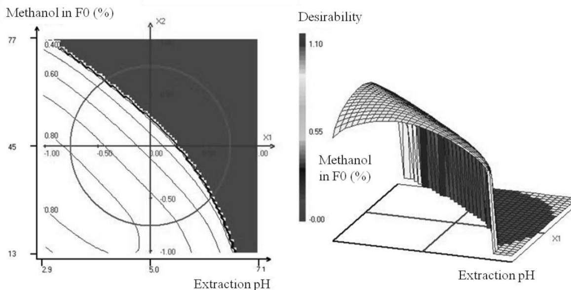
Figure 18. Surface responses (two dimensions on the left and three dimensions on the right) for the recoveries (spiked drinking water) obtained with both RPLC and HILIC methods ( F_0 volume set at 1.5 mL).
