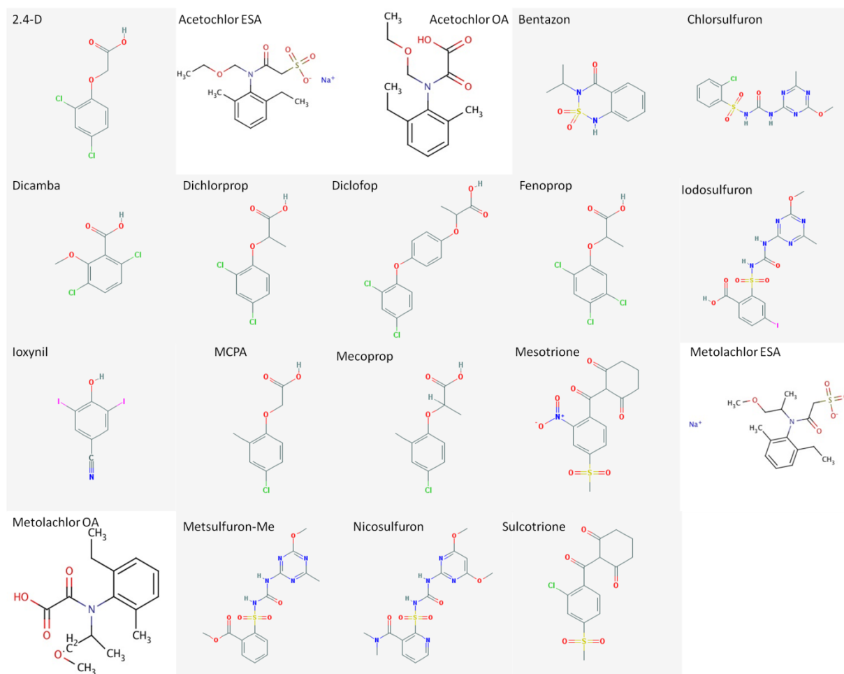
Figure 56. Molecular structure of anionic herbicides ( http://pubchem.ncbi.nlm.nih.gov/ and santa cruz biotechnology, inc. ).
