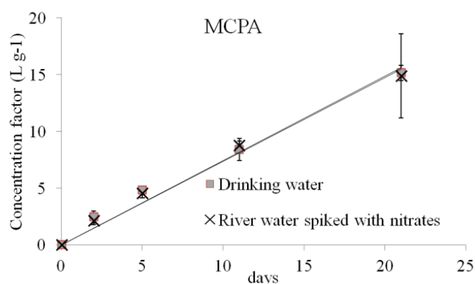
Figure 48. Uptake of MCPA in POCIS-MAX for drinking water (squares) and river water (crosses) spiked with 50 \text{ mg L}^{-1} of nitrate (bars represent the standard deviation, n=3 ).
