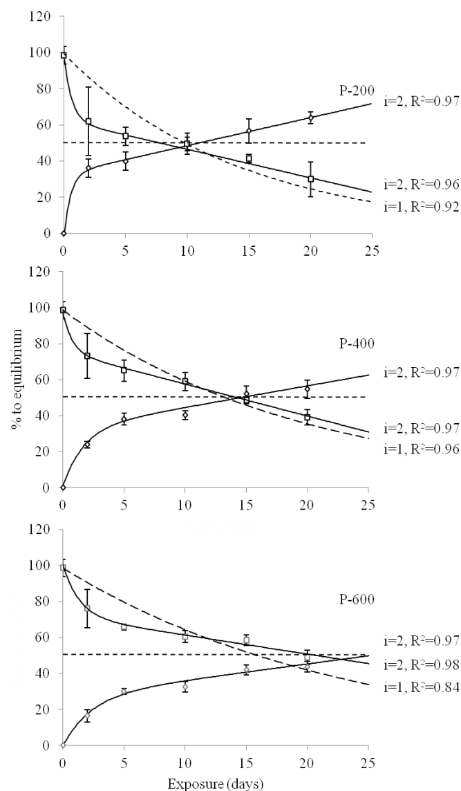
Figure 45. Uptakes and releases of DIA and DIA-d5 for POCIS containing 200, 400 and 600 mg of sorbent (P-200, P-400 and P-600). Monophasic ( i=1 ) and biphasic ( i=2 ) desorption modelling ( n=3 , bars=standard deviation).
