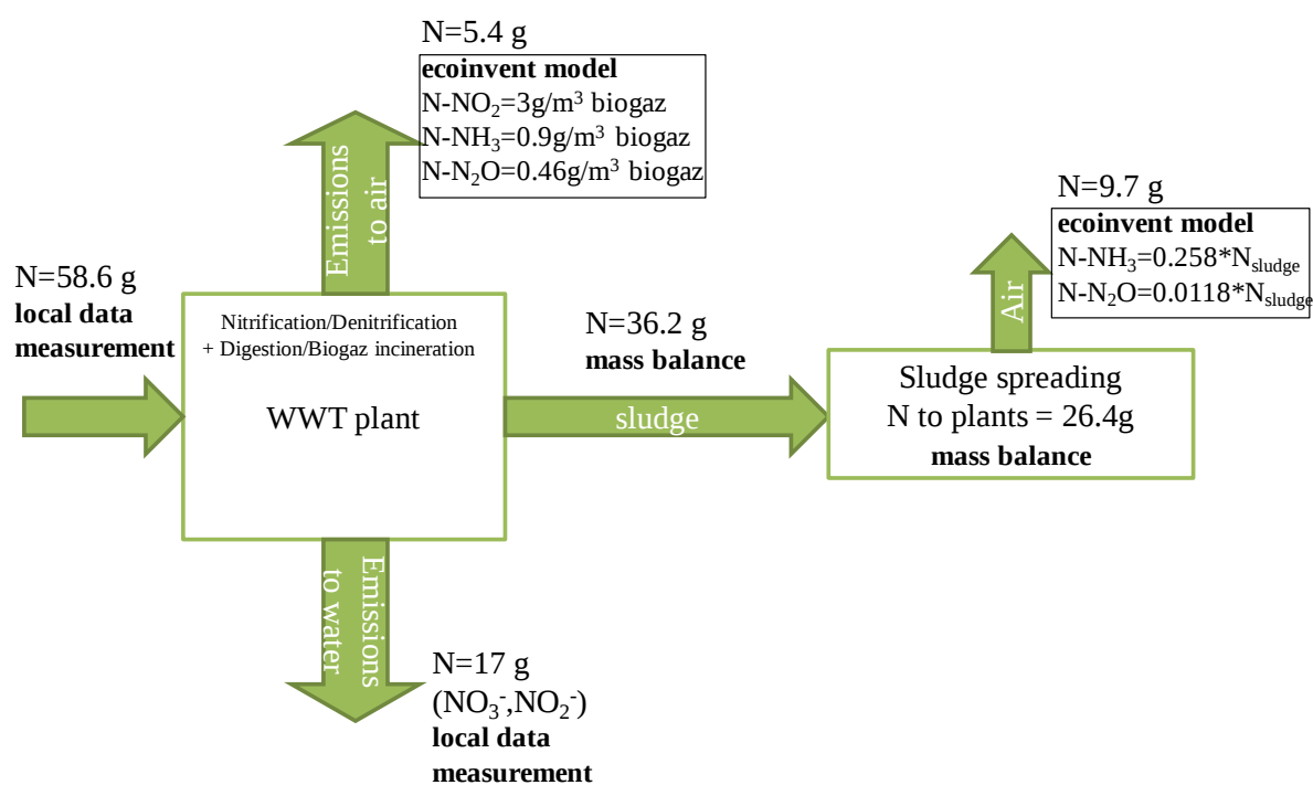
Figure C-7. Nitrogen mass balance in WWT
