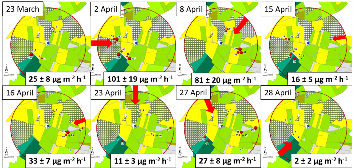
Figure 35: N 2 O fluxes (numbers in \mu\text{g N-N}_2\text{O m}^{-2} \text{ h}^{-1} ) measured by the fast-box on the different sites during the 8 days of measurements. The mean value for each day is recorded. Red arrows show the prevailing wind direction, with the size of the arrow proportional to wind speed.
