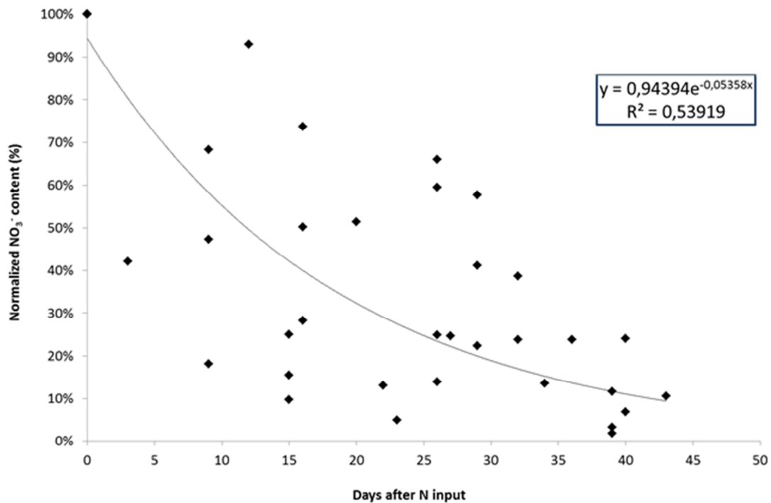
Figure 38: Soil nitrate content (0-20 cm depth) for all sampling date as a function of time following fertilization. The content is normalized by the nitrate content on the day of fertilization. The equation and the line show the function used to account for nitrate consumption over time.
