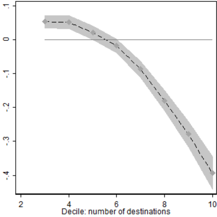
Figure 2.3: Estimated Elasticities
