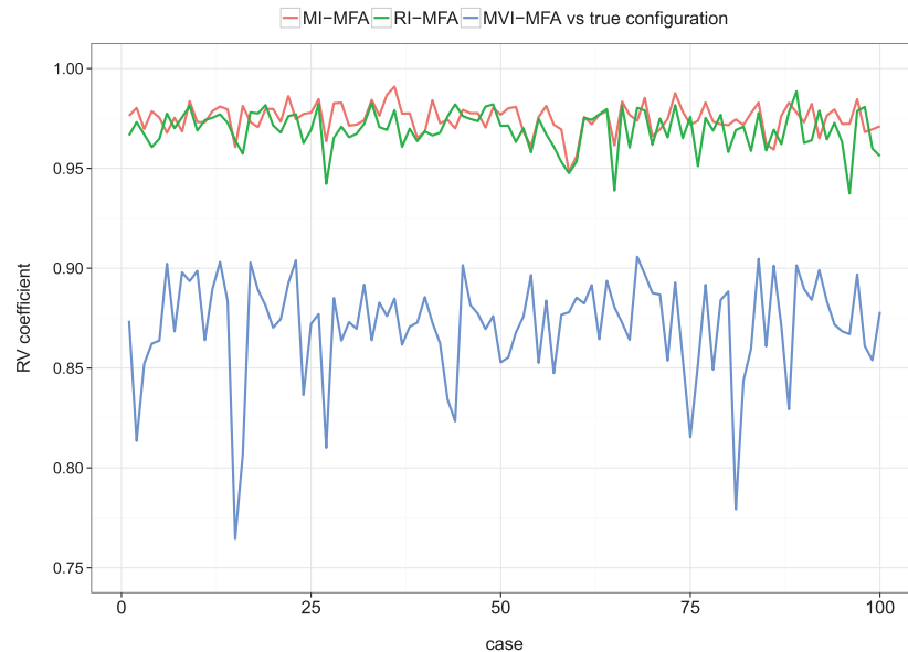
Fig. 8 Performance on NCI-60 data. RV coefficient between the configuration obtained by MFA on the complete dataset and either MI-MFA (red line), RI-MFA (green line) or MVI-MFA (blue line) on the incomplete dataset. The results shown are the mean RV coefficients for the 50 two-dimensional configurations as a function of the cases according to the scenario represented in Table 2. The discrete RV values are joined by lines for ease of understanding
