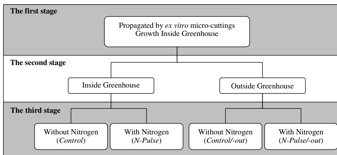
Fig. 3.30 : Scheme of plant preparation during the experiment period 2011. The first stage (August 2009 to 3 November 2010) three branches of plants were prepared inside greenhouse. The second stage (3 November 2010-15 February 2011) separated plants into two groups during late autumn to winter: inside greenhouse group, and outside greenhouse group. The third stage (15 February 2011), the started experiment were moved and placed both groups of plants in same greenhouse with the solution recirculation system. Then, divided the inside greenhouse group into two sub-groups: without (Control) and with N supply (N-Pulse), and also divided the outside greenhouse group into two sub-groups: without (Control/-out) and with N supply (N-Pulse/-out).
