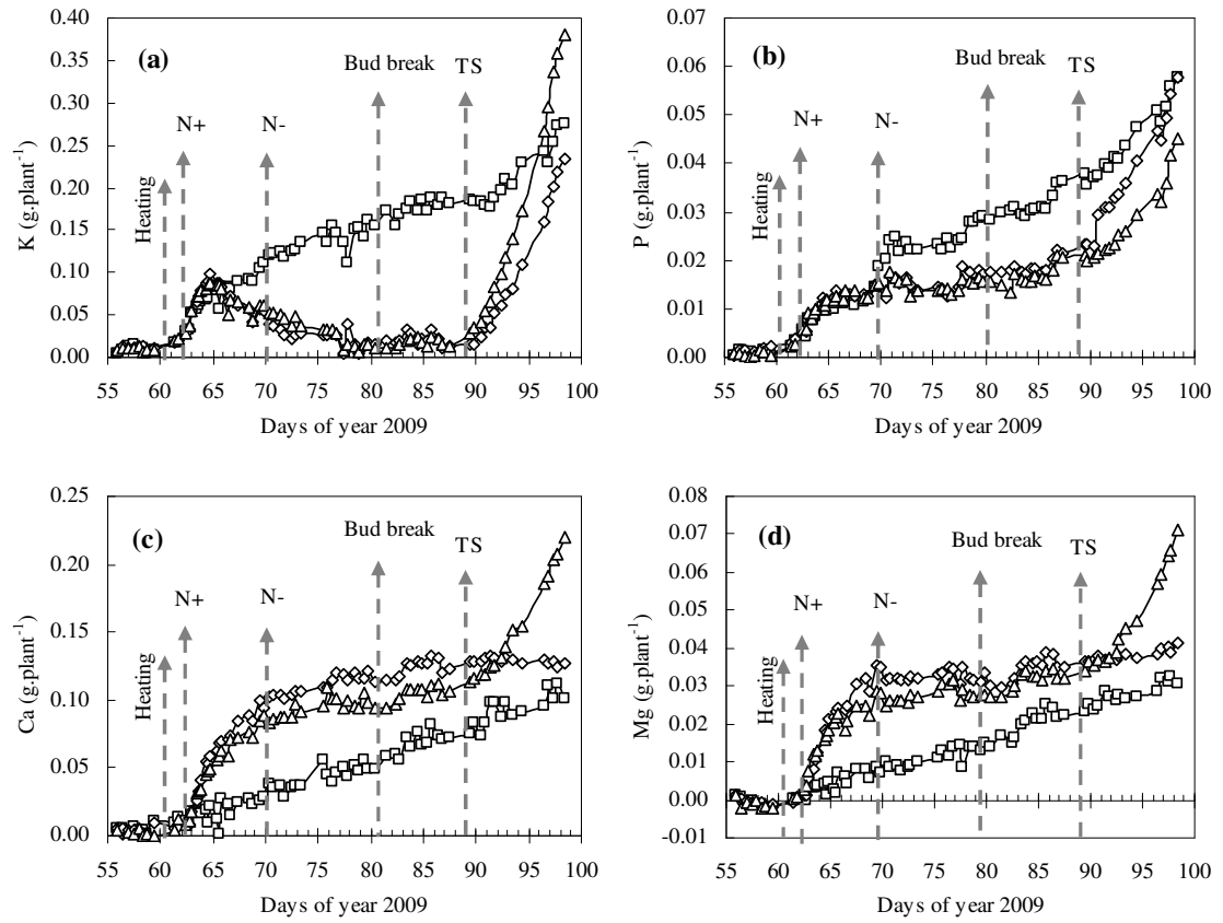
Fig. 3.13 : Cumulated potassium (a), phosphorus (b), calcium (c), and magnesium (d), ( \text{g.plant}^{-1} ) taken up by the one-year scion poplar during the experiment period 2009 in Control ( \square ), N-Pulse ( \diamond ), and N-Supply ( \Delta ) conditions. The arrows represent the time of increase temperature in greenhouse, start experiment during nitrate solution supply in N-Pulse and N-Supply treatments (N+), first time change solution without nitrate to N-Pulse treatment (-N), bud break period (Bud break), and start transpiration (TS), respectively
